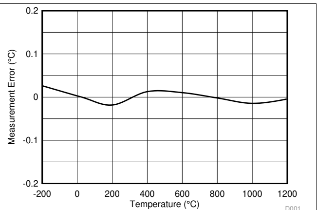
Figure 76. Temperature Measurement Error vs T_{(TC)}
