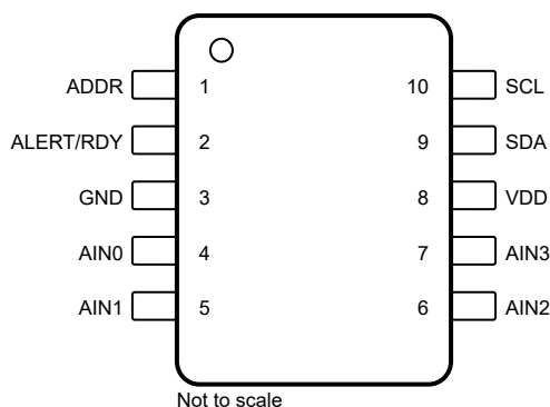
Figure 4-2. DYN and DGS Packages, 10-Pin (Top View)
