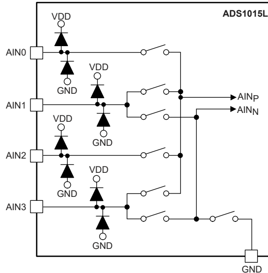
Figure 7-3. Input Multiplexer
