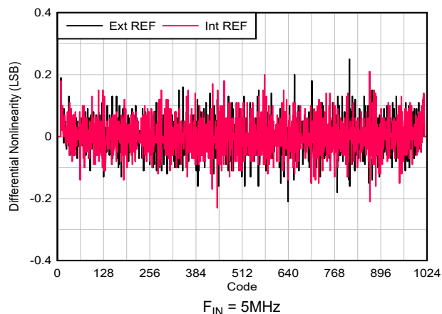
Figure 5-37. DNL vs ADC Code
