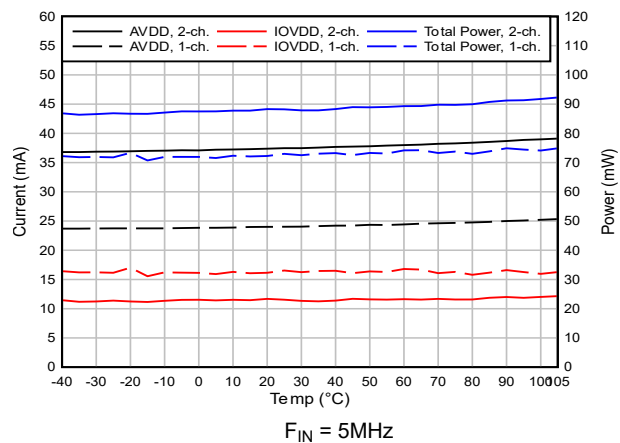
Figure 6-53. Current vs Temperature
