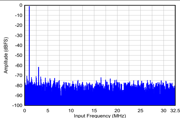
Figure 6-19. Single Tone FFT at F_{IN} = 1\text{MHz}
