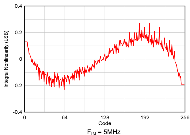
Figure 6-49. INL vs ADC Code
