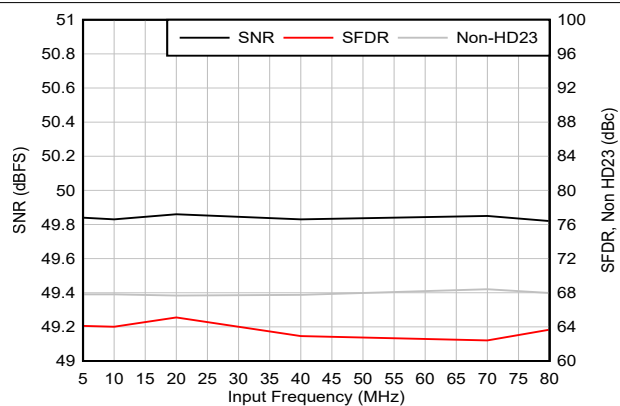
Figure 6-24. AC Performance vs Input Frequency
