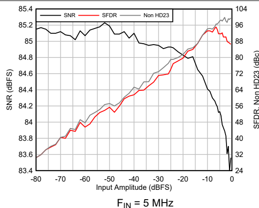
Figure 5-12. AC Performance Vs Input Amplitude
