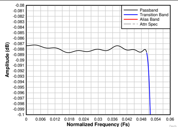
Figure 7-26. Decimation by 8 Filter Passband Ripple Response
