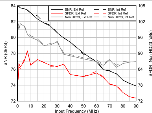
Figure 5-10. AC Performance Vs Input Frequency
