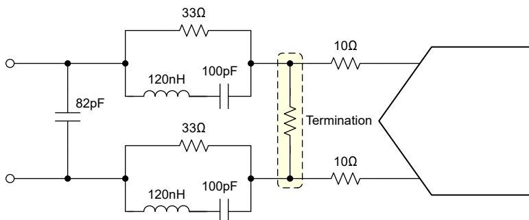
Figure 7-5. Sampling Glitch Filter for Input Frequencies from 30MHz to 70MHz
