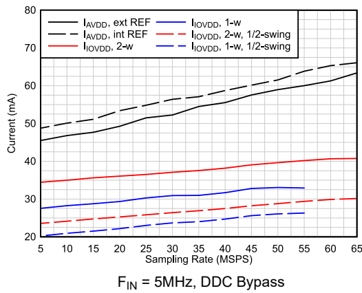
Figure 5-25. Current vs Sampling Rate
