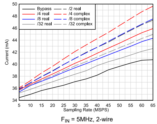
Figure 5-26. I_{IOVDD} Current vs Decimation
