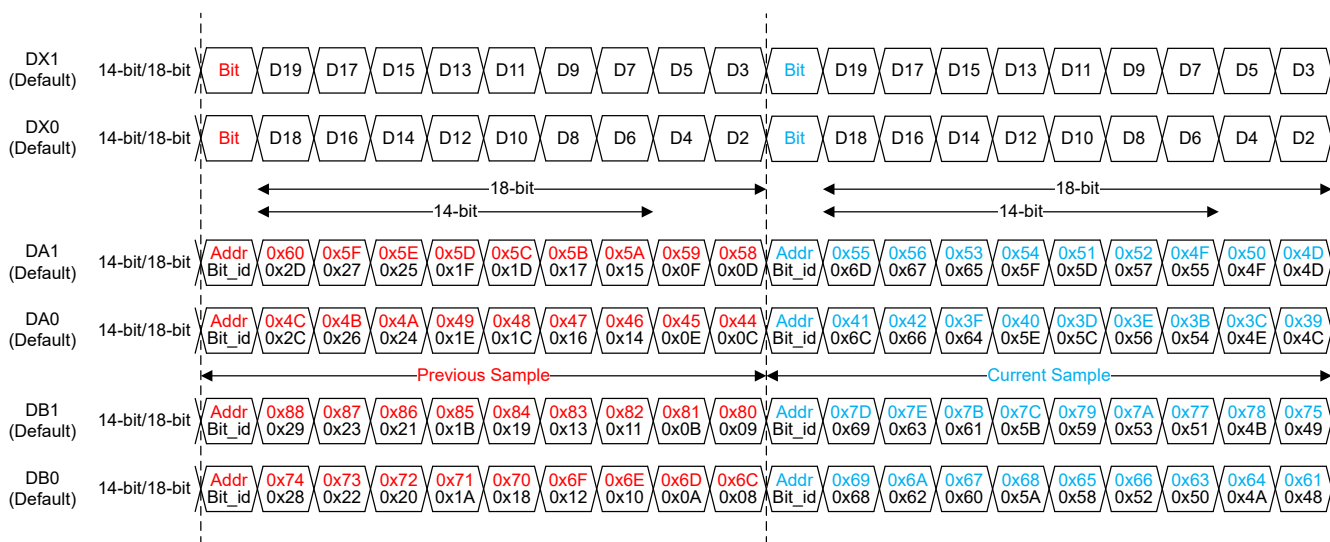
Figure 7-13. Default Bit Mapping for 2-wire, 14-bit/18-bit
