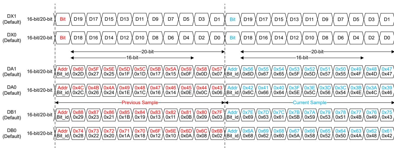
Figure 7-14. Default Bit Mapping for 2-wire, 16-bit/20-bit
