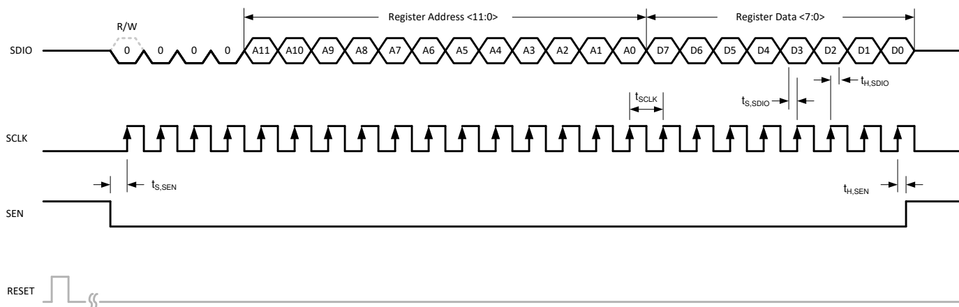
Figure 8-43. Serial Register Write Timing Diagram
