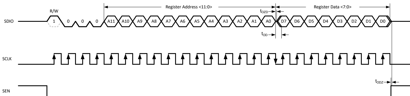
Figure 8-44. Serial Register Read Timing Diagram
