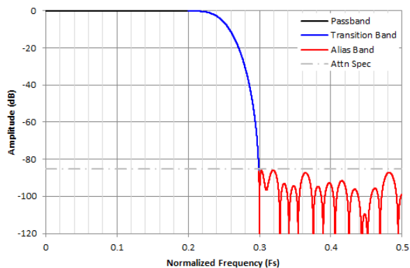
Figure 8-23. Complex Decimation by 2 Filter Response
