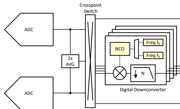
Figure 8-53. NCO Block Diagram
