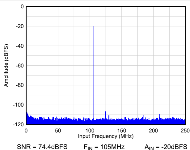
Figure 8-73. FFT - no AVG
