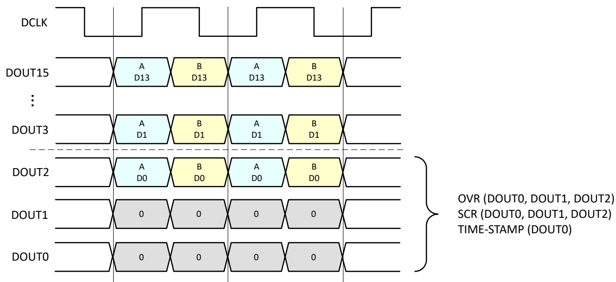
Figure 8-55. Output data format in DDR LVDS mode
