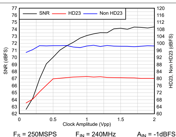
Figure 8-14. AC vs Clock Amplitude
