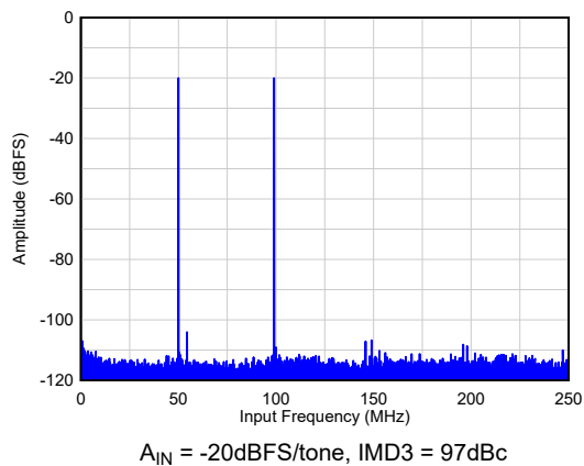
Figure 6-39. Two Tone FFT at F_{IN} = 445/455\text{MHz}
