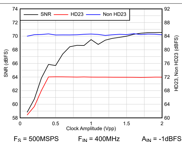
Figure 8-12. AC vs Clock Amplitude
