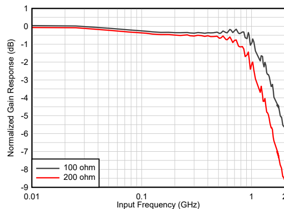
Figure 8-6. Full power input bandwidth for 100\Omega and 200\Omega internal termination
