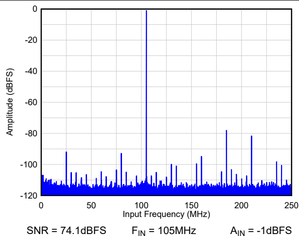
Figure 8-71. FFT - no AVG
