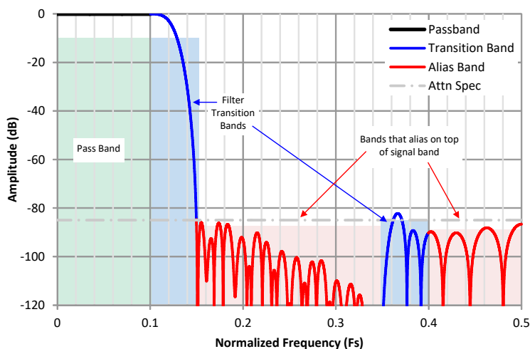
Figure 8-22. Interpretation of the Decimation Filter Plots
