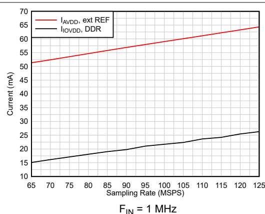
Figure 6-24. Current vs Sampling Rate
