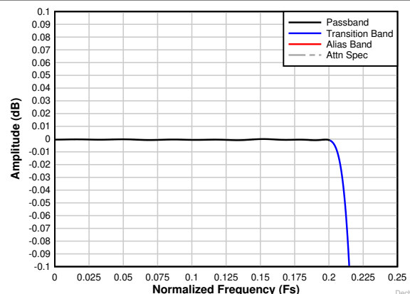
Figure 8-21. Decimation by 2 complex passband ripple response
