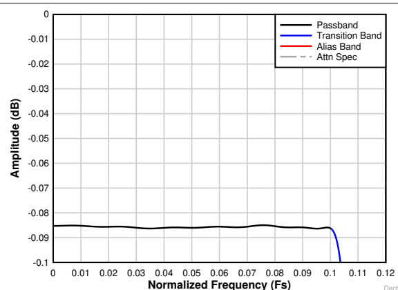
Figure 8-23. Decimation by 4 complex passband ripple response
