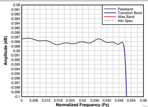
Figure 8-25. Decimation by 8 complex passband ripple response
