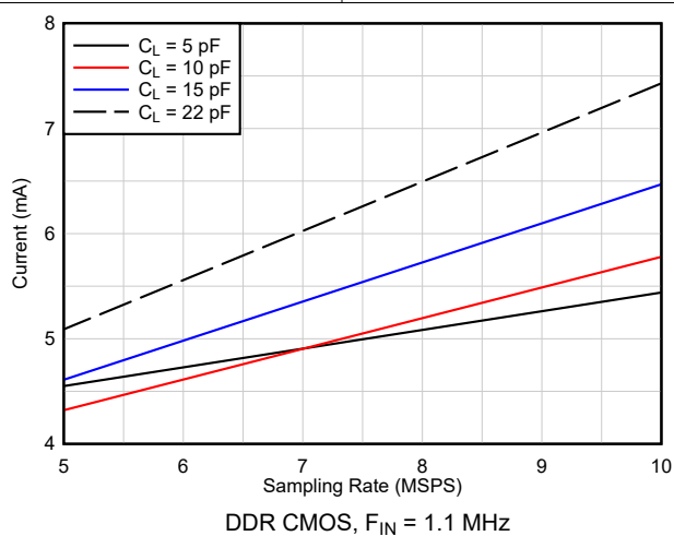
Figure 6-17. I_{OVDD} Current vs Load Capacitance
