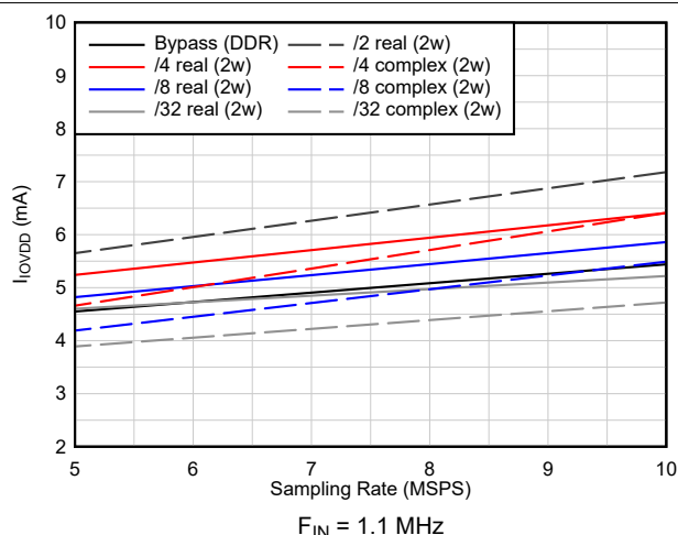
Figure 6-16. I_{OVDD} Current vs Decimation
