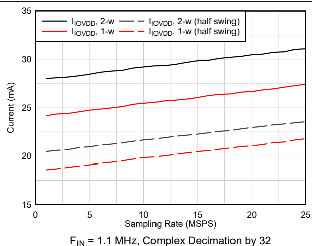
Figure 6-39. I_{IOVDD} Current vs Interface
