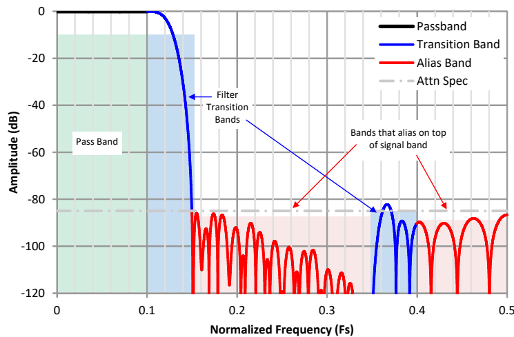
Figure 8-22. Interpretation of the Decimation Filter Plots
