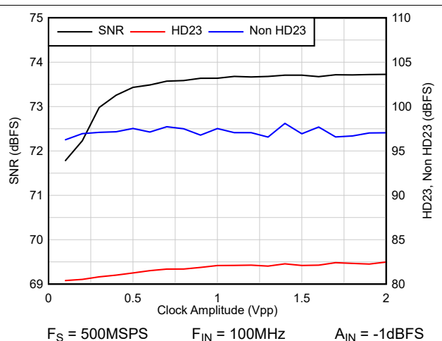
Figure 9-3. SNR vs Clock Amplitude
