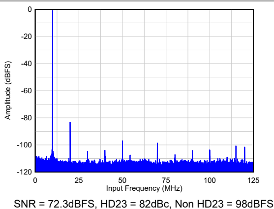
Figure 6-5. Single Tone FFT at F_{IN} = 240\text{MHz}
