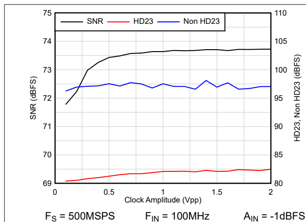
Figure 8-11. AC vs Clock Amplitude
