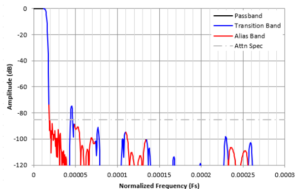
Figure 8-51. Complex Decimation by 32768 Filter Response
