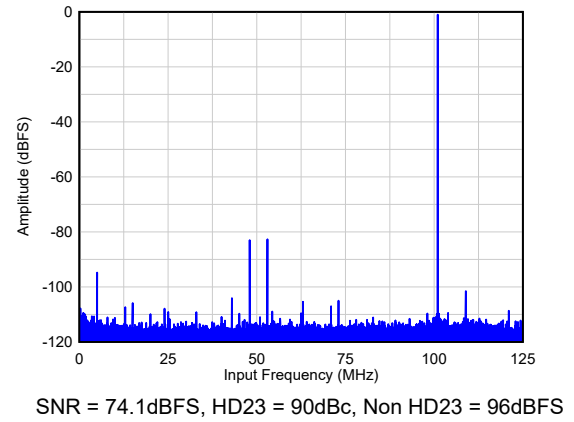
Figure 6-2. Single Tone FFT at F_{IN} = 101\text{MHz}
