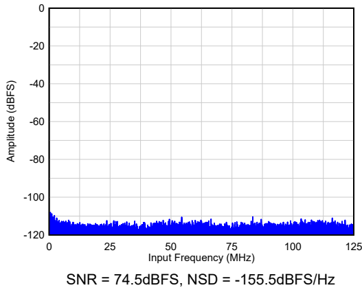
Figure 6-1. Idle Channel Noise
