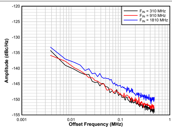
Figure 8-10. Amplitude Noise Examples
