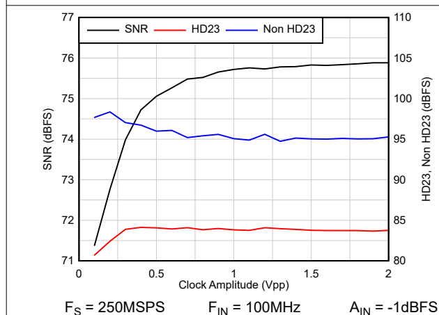
Figure 8-13. AC vs Clock Amplitude
