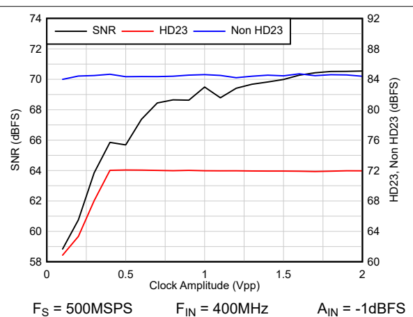
Figure 8-12. AC vs Clock Amplitude
