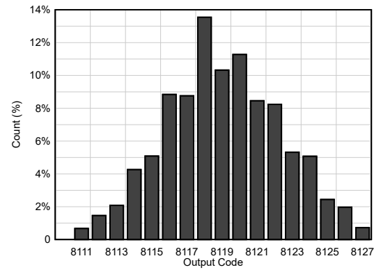
Figure 6-52. DC Offset Histogram
