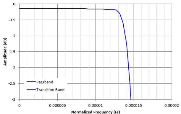
Figure 8-52. Decimation by 32768 Passband Ripple Response
