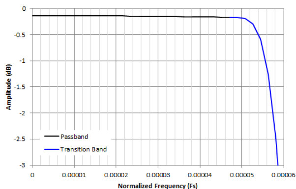
Figure 8-48. Decimation by 8192 Passband Ripple Response
