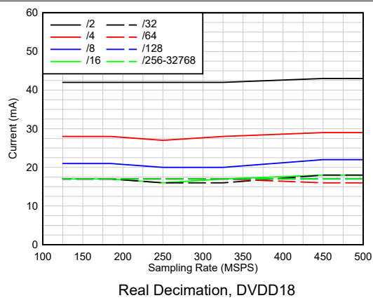
Figure 6-55. Current vs Sampling Rate
