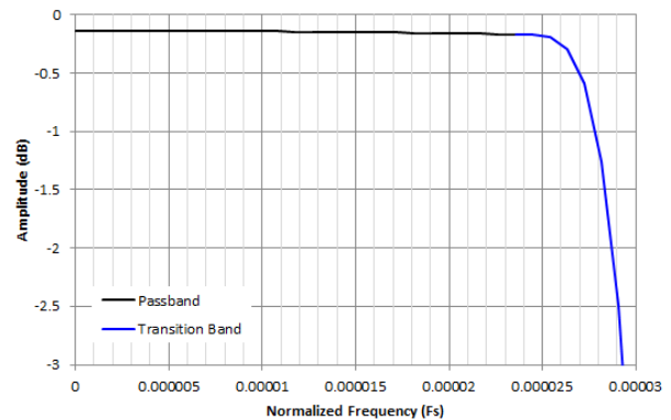
Figure 8-50. Decimation by 16384 Passband Ripple Response
