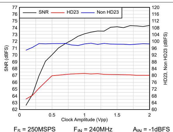
Figure 8-14. AC vs Clock Amplitude
