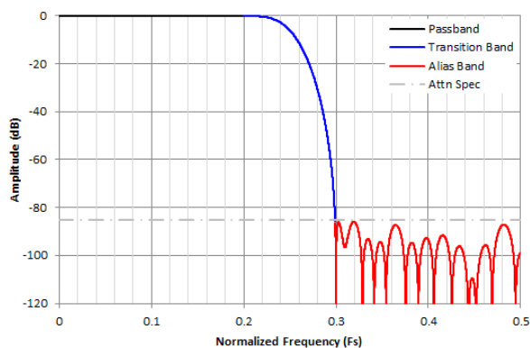
Figure 8-23. Complex Decimation by 2 Filter Response
