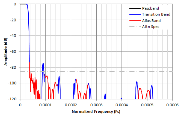
Figure 8-49. Complex Decimation by 16384 Filter Response
