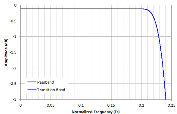
Figure 8-24. Decimation by 2 Passband Ripple Response
