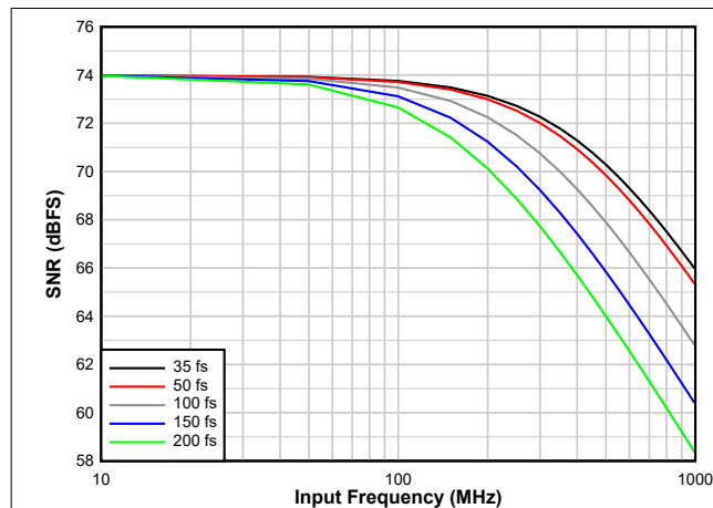
Figure 9-2. SNR vs T_{\text{Jitter}} vs F_{\text{IN}}
