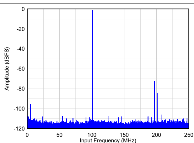
Figure 8-69. FFT: F_{IN} = 105\text{MHz} , low latency mode
