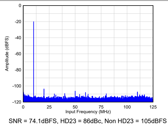
Figure 6-6. Single Tone FFT at F_{IN} = 240\text{MHz} , A_{IN} = -20\text{dBFS}
