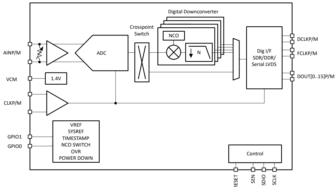
Figure 8-1. Block Diagram
