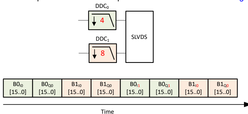
Figure 8-21. Unequal Decimation Factors
