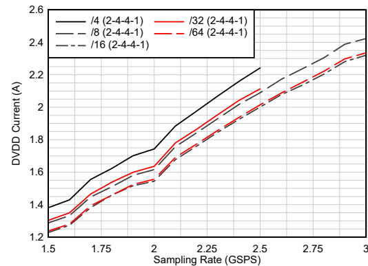
Figure 5-46. Current vs Sampling Rate vs Complex Decimation
