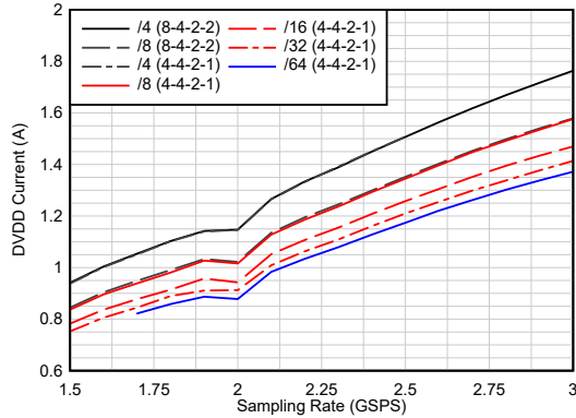
Figure 5-43. Current vs Sampling Rate vs Real Decimation
