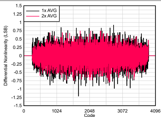
Figure 5-39. DNL vs Code
