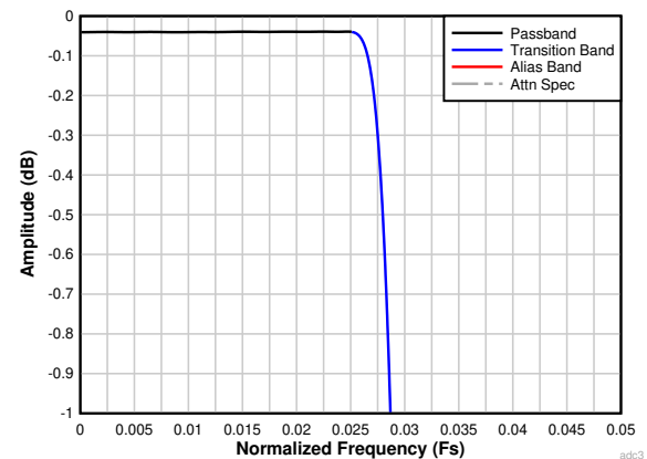
Figure 6-29. Decimation by 16 Passband Ripple Response
