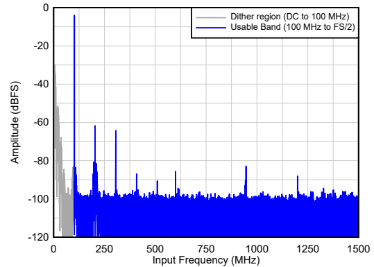
Figure 5-2. Single Tone FFT at F_{IN} = 100 MHz
