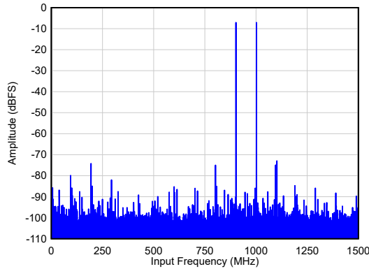
IMD3 = 68 dBc A_{IN} = -7\text{ dBFS/tone} , 1x AVG, Dither = DIS Figure 5-19. Two Tone FFT at F_{IN} = 900/1000\text{ MHz}
