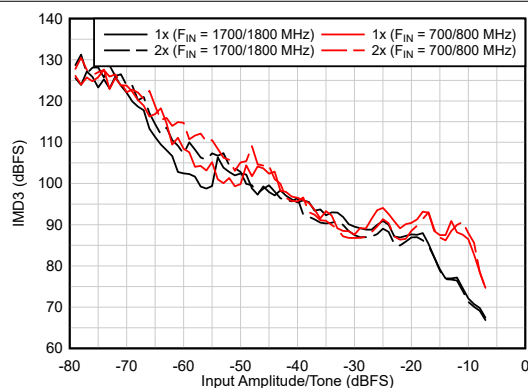
Figure 5-29. IMD3 Performance vs A_{IN}
