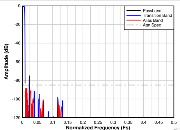
Figure 6-32. Complex Decimation by 64 Filter Response
