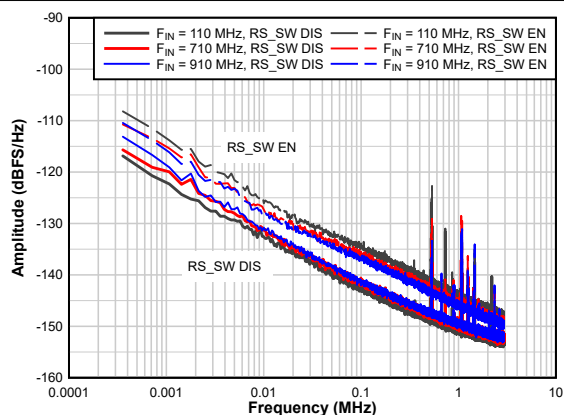
Figure 6-10. Amplitude Noise vs Input Frequency
