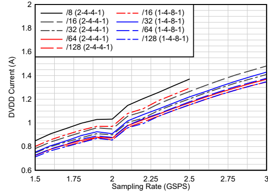
Figure 5-44. Current vs Sampling Rate vs Real Decimation
