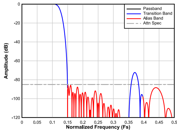
Figure 6-24. Complex Decimation by 4 Filter Response
