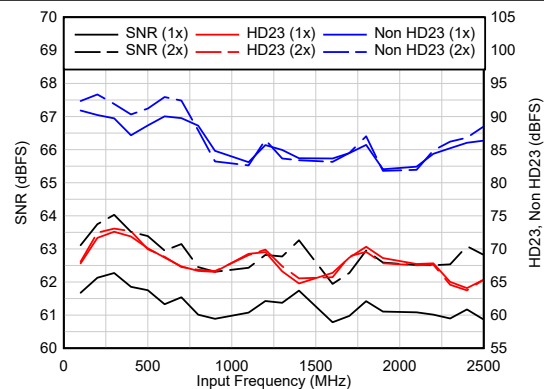
A_{IN} = -4\text{ dBFS} , Dither = EN Figure 5-24. AC Performance vs F_{IN}
