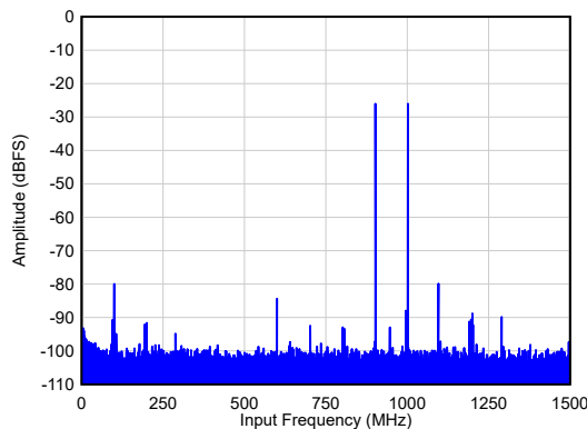
IMD3 = 54 dBc A_{IN} = -26\text{ dBFS/tone} , 1x AVG, Dither = DIS Figure 5-21. Two Tone FFT at F_{IN} = 900/1000\text{ MHz}
