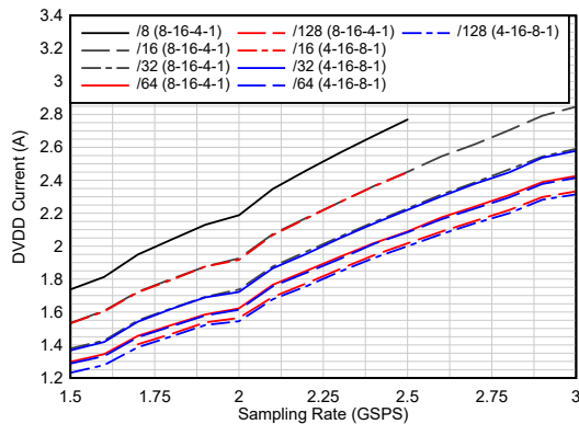
Figure 5-45. Current vs Sampling Rate vs Complex Decimation
