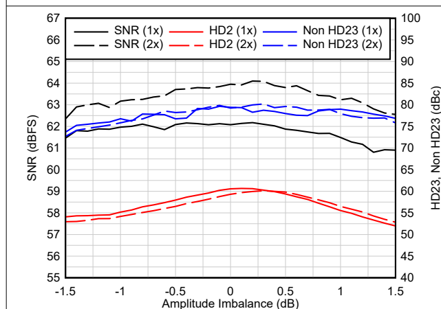
Figure 6-5. Amplitude Imbalance - 3.0 GSPS
