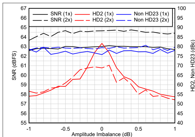
Figure 6-3. Amplitude Imbalance - 2.6 GSPS
