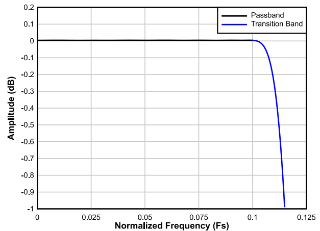
Figure 6-25. Decimation by 4 Passband Ripple Response
