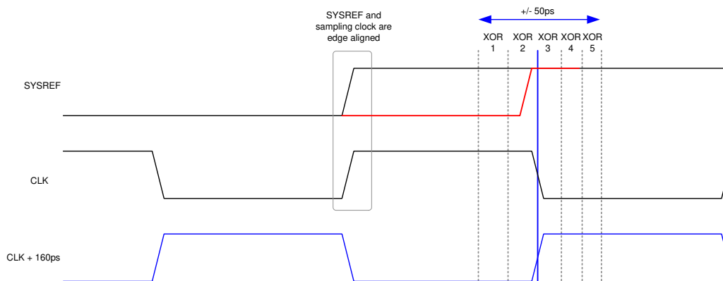
Figure 6-22. Detection of SYSREF Transition within Capture Window
