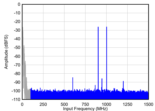
IMD3 = 71 dBc A_{IN} = -26\text{ dBFS/tone} , 1x AVG, Dither = EN Figure 5-22. Two Tone FFT at F_{IN} = 900/1000\text{ MHz}
