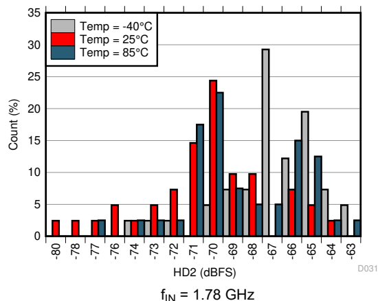
Figure 6-55. HD2 Histogram at AVDD19 = 1.8 V
