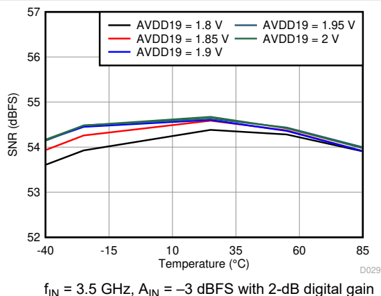
Figure 6-53. Signal-to-Noise Ratio vs. AVDD19 Supply and Temperature
