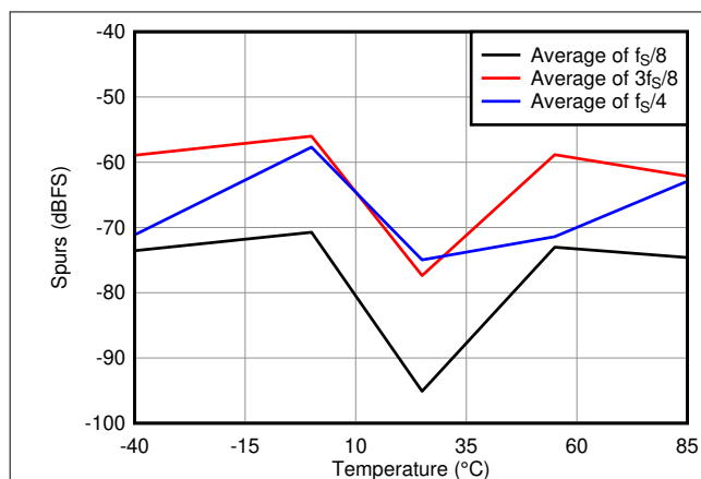
Figure 9-7. Offset Corrector Block Frozen at Room Temperature
