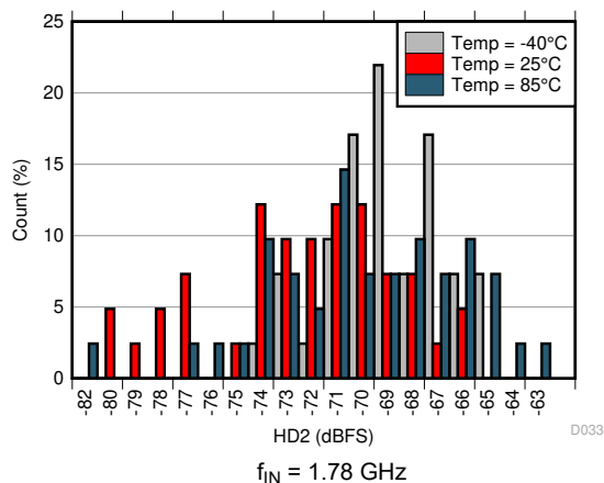
Figure 6-57. HD2 Histogram at AVDD19 = 2.0 V
