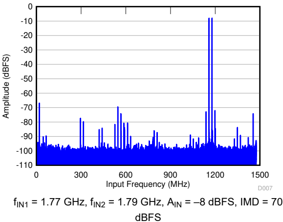
Figure 6-19. FFT for Two-Tone Input Signal (–8 dBFS)
