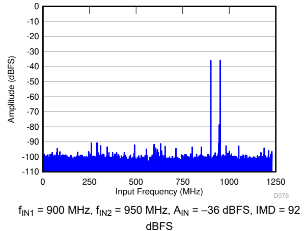
Figure 6-18. FFT for Two-Tone Input Signal (–36 dBFS, f_s = 2457.6 \text{ MSPS} )
