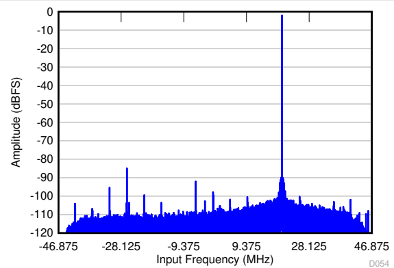
Figure 6-78. FFT in 32x Decimation (Complex Output)
