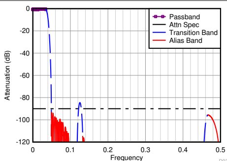
Figure 8-29. Divide-by-12 Filter Response
