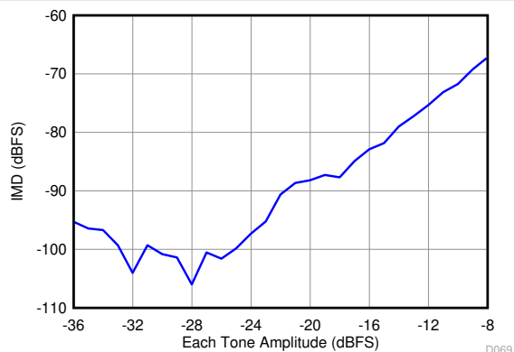
Figure 6-36. Intermodulation Distortion vs. Input Amplitude (3490 MHz and 3510 MHz, f_s = 2457.6 MSPS)
