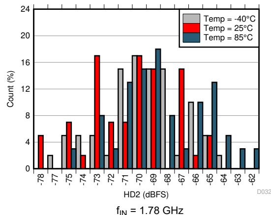
Figure 6-56. HD2 Histogram at AVDD19 = 1.9 V
