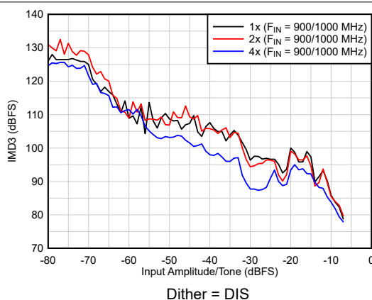
Figure 6-36. IMD3 Performance vs A_{IN}
