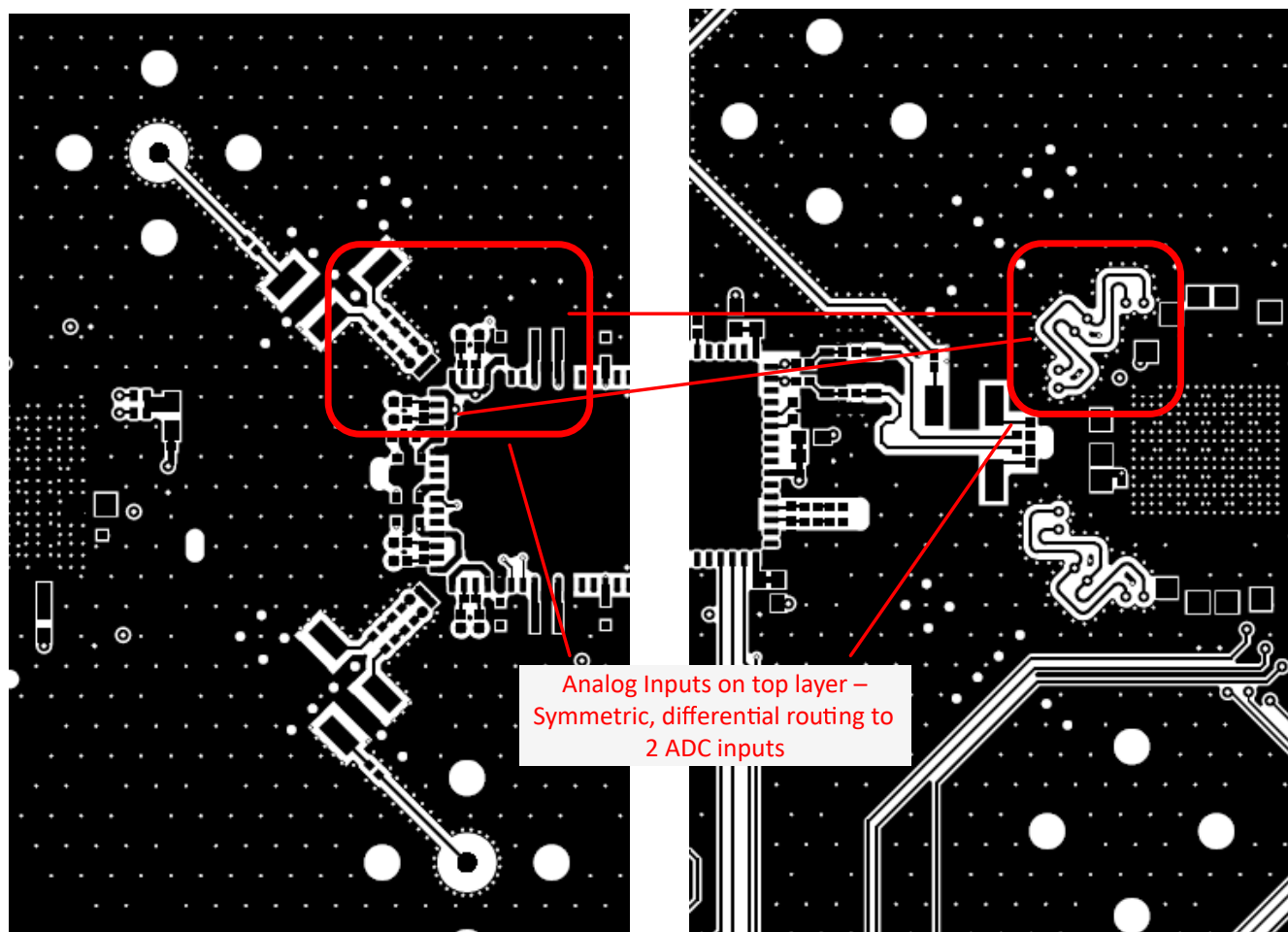
Figure 8-8. Layout example for 4x AVG: ADC32RF5x EVM
