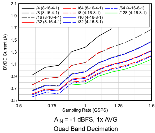
Figure 6-55. Current vs Sampling Rate vs Complex Decimation
