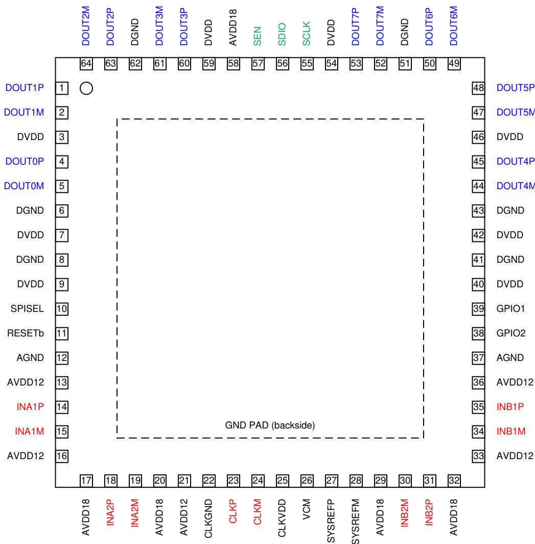
Figure 5-1. RTD (VQFNP) Package, 64 Pin (Top View)
