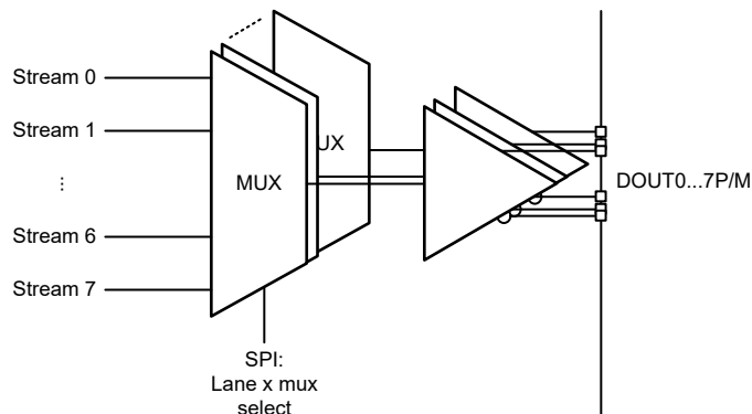
Figure 7-40. SERDES output mux for DOUT0
