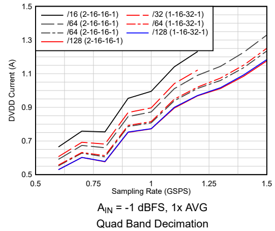
Figure 6-56. Current vs Sampling Rate vs Complex Decimation
