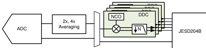
Figure 7-20. Digital Decimation Filter Options
