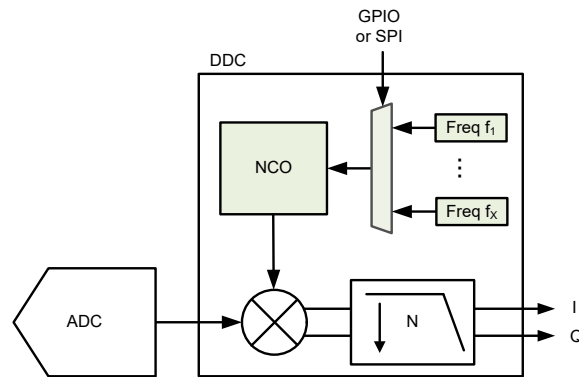
Figure 7-35. NCO Block Diagram
