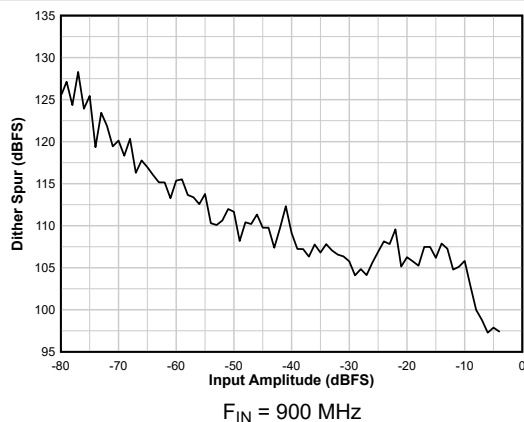
Figure 6-31. Dither Spur vs A_{IN}
