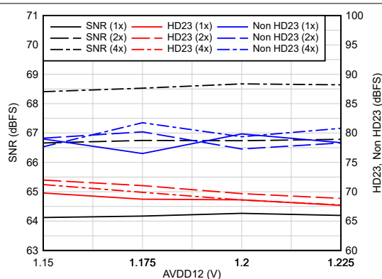
Figure 6-41. AC Performance vs AVDD12
