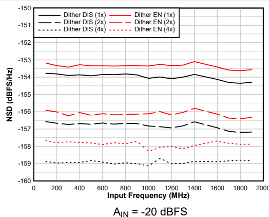
Figure 6-32. NSD Performance vs F_{IN}
