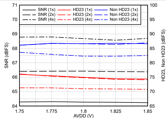
Figure 6-40. AC Performance vs AVDD18
