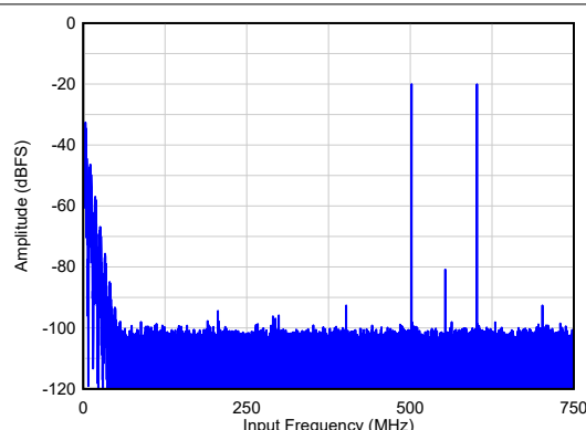
Figure 6-22. Two Tone FFT at F_{IN} = 900, 1000 MHz
