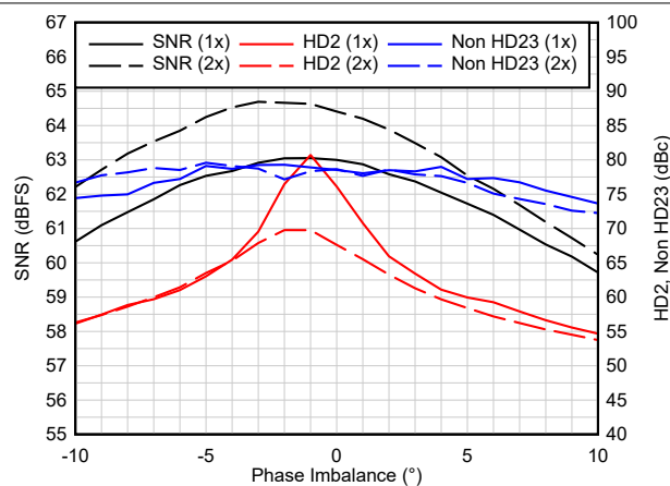
Figure 7-3. Amplitude Imbalance vs SNR
