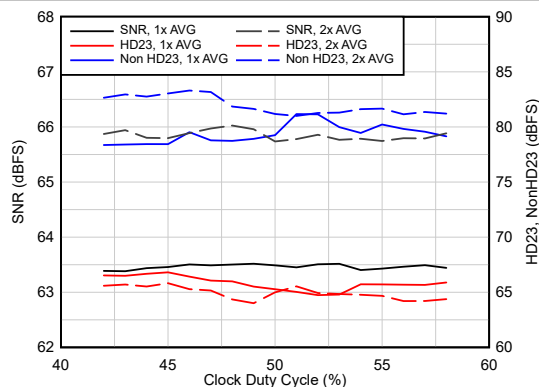
Figure 6-39. AC Performance vs Clock Duty Cycle
