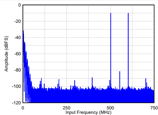
Figure 6-26. Two Tone FFT at F_{IN} = 900, 1000\text{ MHz}
