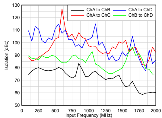
Figure 6-38. Isolation vs Input Frequency
