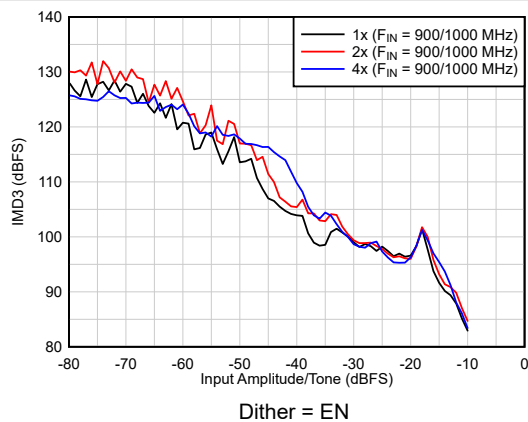
Figure 6-37. IMD3 Performance vs A_{IN}
