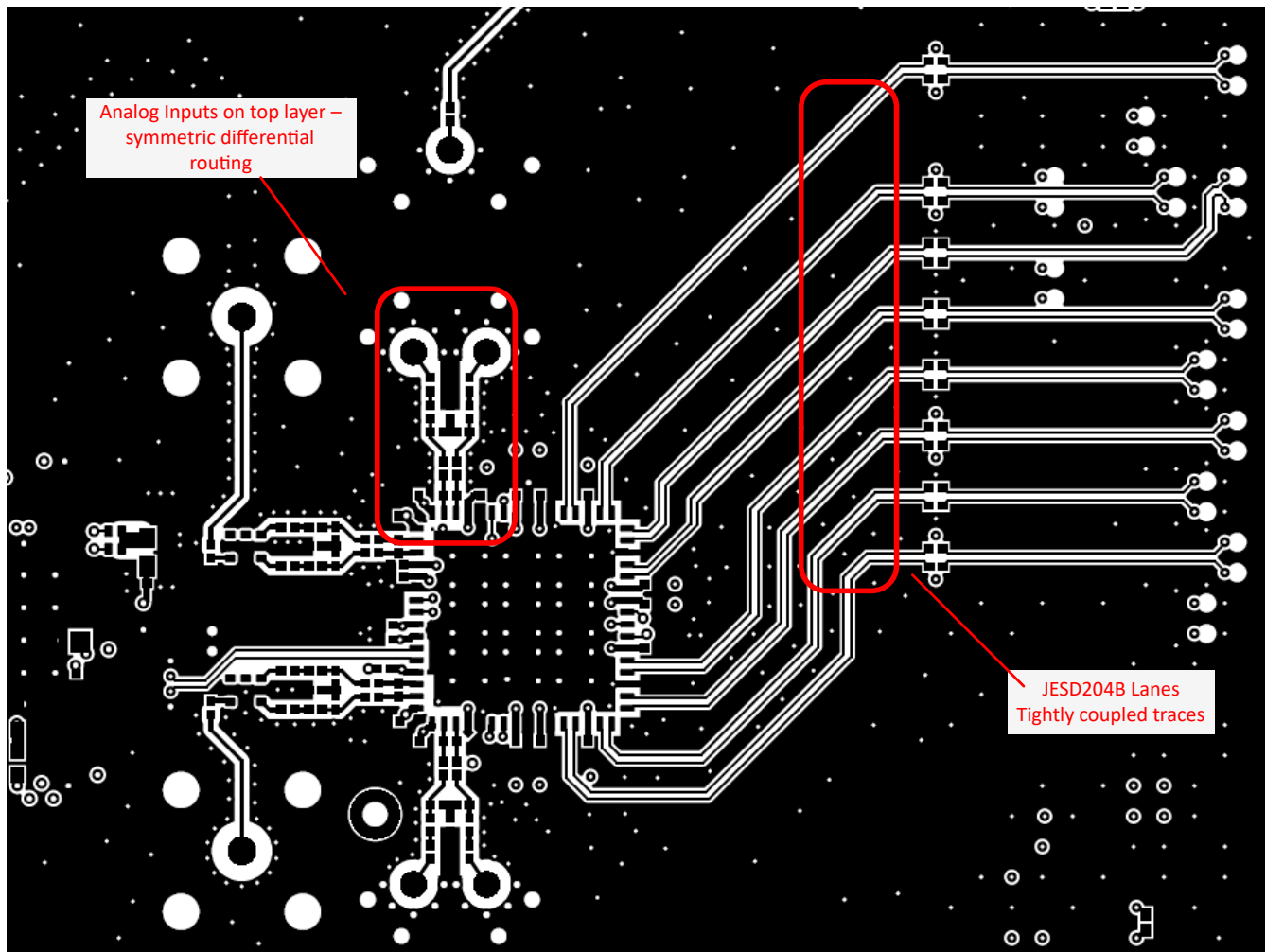
Figure 8-7. Layout example: top layer of ADC32RF5x EVM
