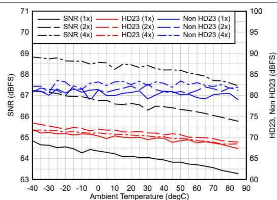
Figure 6-42. AC Performance vs Temperature
