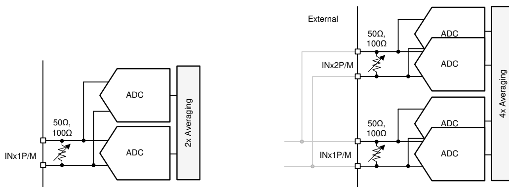
Figure 7-42. Internal digital averaging (left: 2x, right: 4x)
