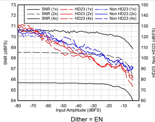
Figure 6-34. AC Performance vs A_{IN}
