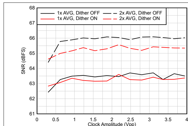
Figure 7-9. SNR vs Clock Amplitude ( F_{IN} = 900 MHz)
