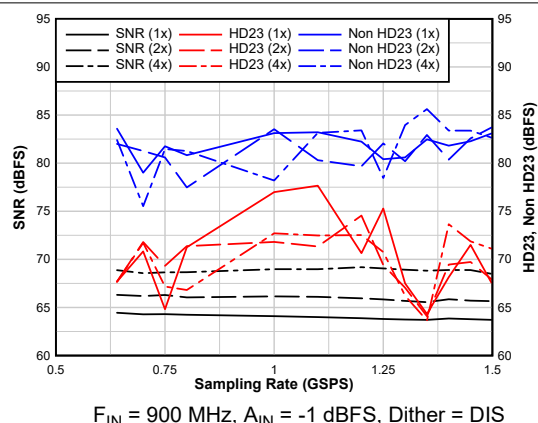
Figure 6-35. AC Performance vs F_S
