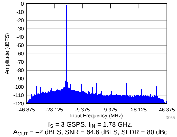
Figure 58. FFT in 32X Decimation (Complex Output)
