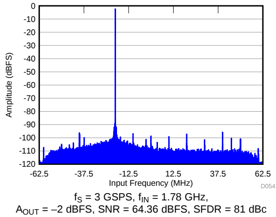
Figure 57. FFT in 24X Decimation (Complex Output)
