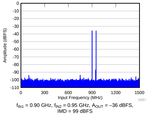
Figure 10. FFT for Two-Tone Input Signal (-36 dBFS)
