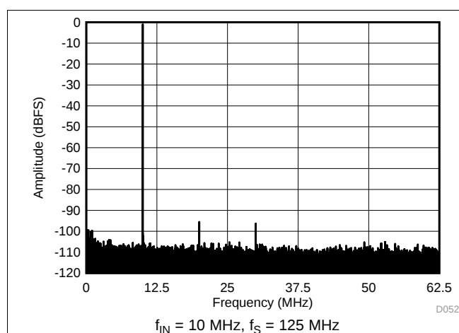
Figure 143. Chopper Off
