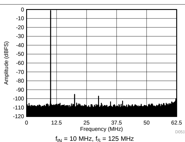
Figure 144. Chopper On
