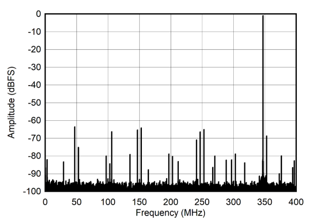
Figure 5-14. Single Tone FFT at 347 MHz and -1dBFS
