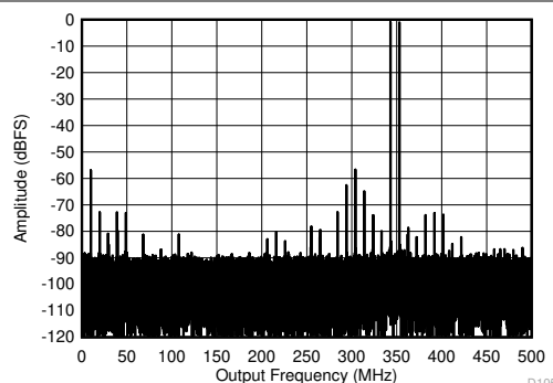
10 MHz tone spacing, -7 dBFS per tone, Low power mode, 1000MSPS Figure 5-72. Two Tone FFT at 348 MHz
