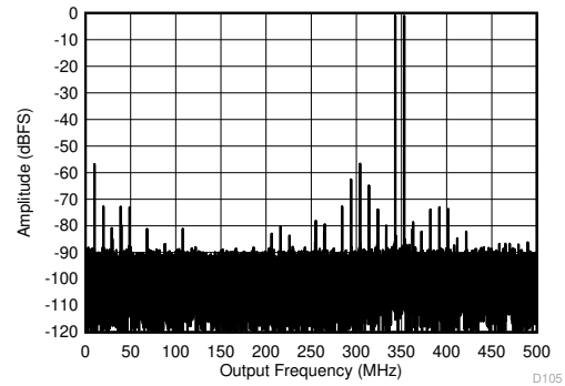
Figure 5-72. Two Tone FFT at 348 MHz 10 MHz tone spacing, -7 dBFS per tone, Low power mode, 1000MSPS
