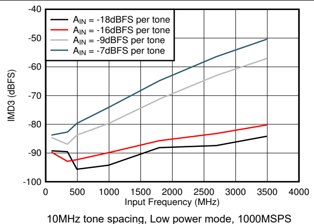
Figure 5-76. IMD3 vs F_{IN}
