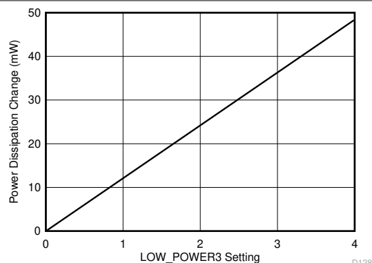
Figure 6-11. Power Dissipation Change vs LOW_POWER3 register setting
