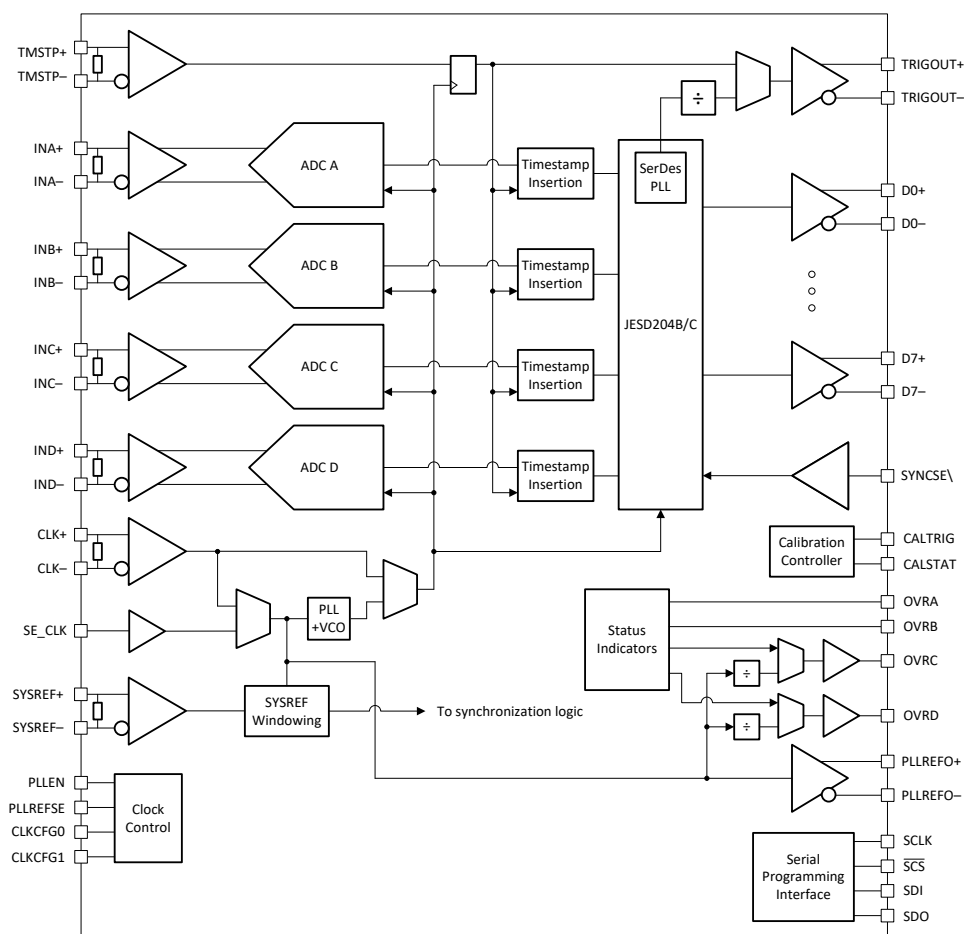
Quad Channel Block Diagram
