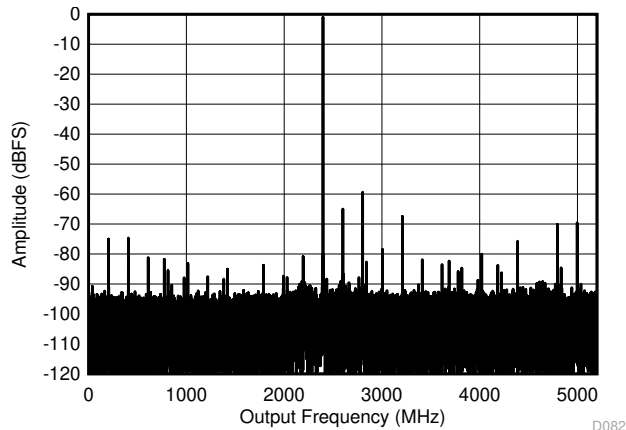
Figure 5-7. DES Mode: Single Tone FFT at 2397MHz
