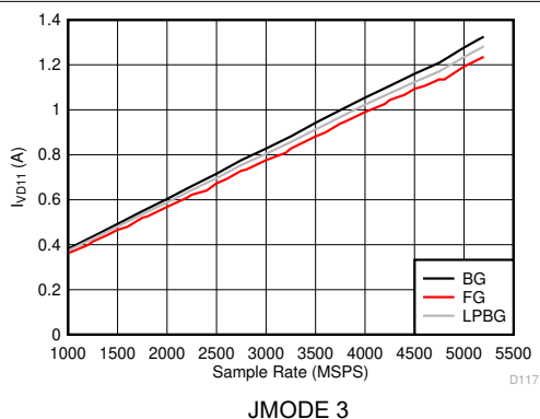
Figure 5-135. Dual Channel Mode: I_{VD11} vs Sample Rate
