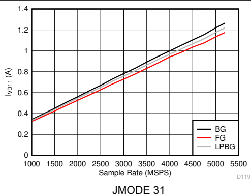
Figure 5-137. Dual Channel Mode: I_{VD11} vs Sample Rate
