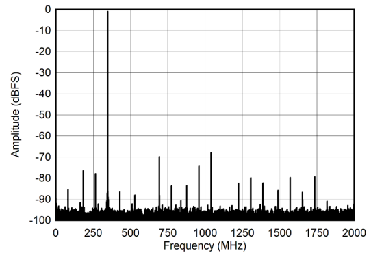
Figure 6-18. Dual Channel Mode: Single Tone FFT at 347 MHz
