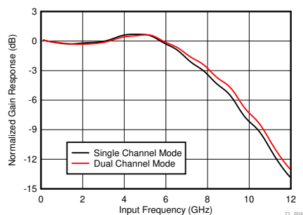
ADC12DJ3200 Measured Input Bandwidth
