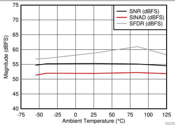
Figure 32. SNR, SINAD, SFDR vs Temperature
