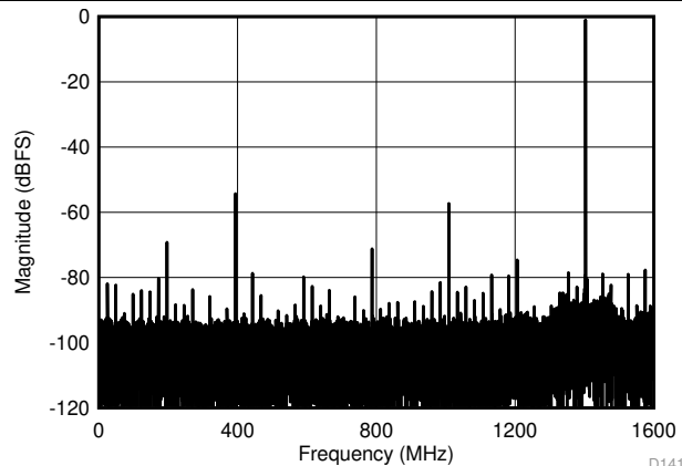
Figure 24. Single-Tone FFT at A_{\text{IN}} = -1\text{ dBFS}
