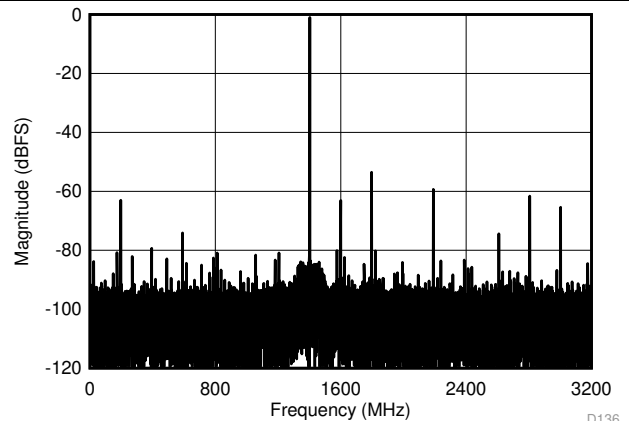
Figure 25. Single-Tone FFT at A_{\text{IN}} = -1\text{ dBFS}
