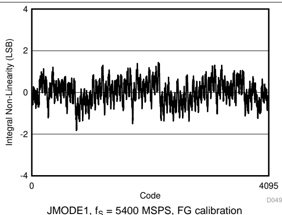
Figure 31. INL vs Code
