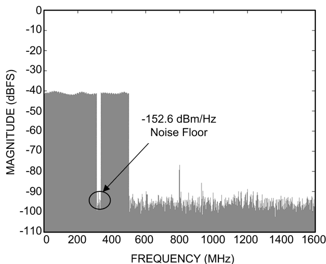
Wideband Performance
