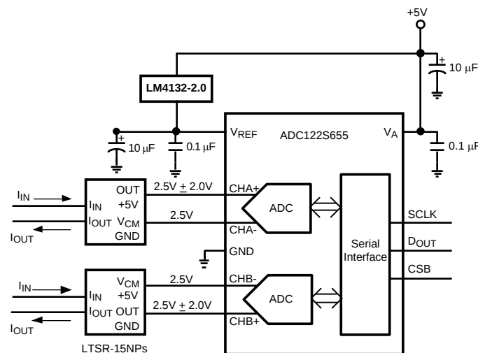
Figure 39. Interfacing the ADC122S655 to a Current Transducer
