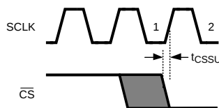
Figure 5. Valid \overline{CS} Assertion Times
