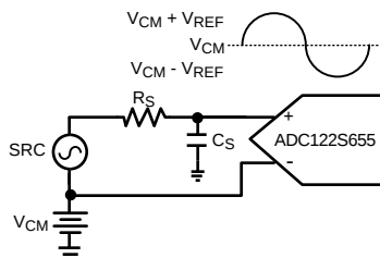
Figure 35. Single-Ended Input
