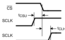
Figure 6. SCLK and \overline{CS} Timing Parameters
