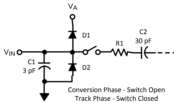
Figure 52. Equivalent Input Circuit
