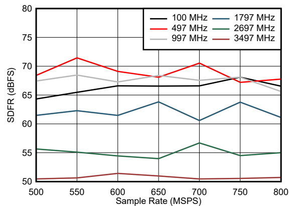
Figure 5-20. SFDR vs Sample Rate
