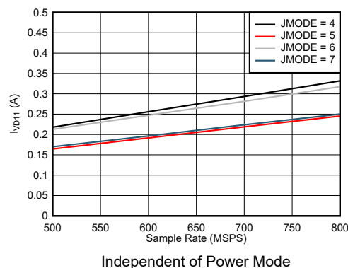
Figure 5-78. Quad Channel, I_{VD11} vs F_S for JMODES 4 - 7
