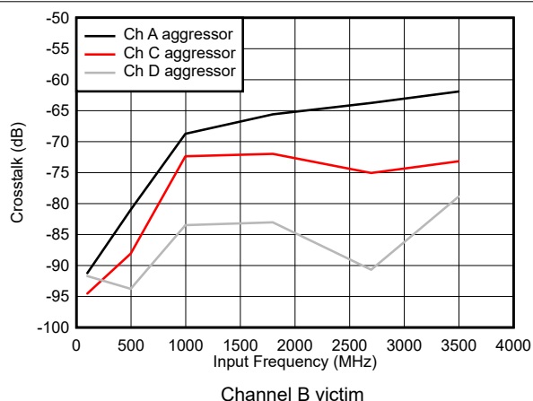
Figure 5-62. Crosstalk vs Input Frequency
