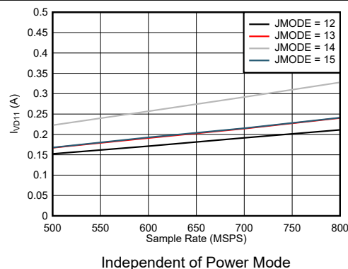
Figure 5-80. Quad Channel, I_{VD11} vs F_S for JMODES 12 - 15
