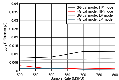
Figure 5-110. Quad Channel, I_{VD11} Change with Calibration Mode
