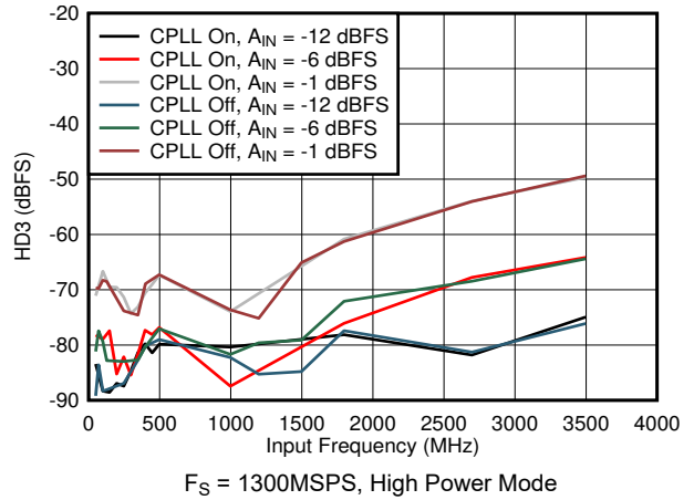
Figure 5-74. HD3 vs Input Frequency, CPLL and Input Amplitude
