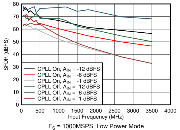
Figure 5-76. SFDR vs Input Frequency, CPLL and Input Amplitude
