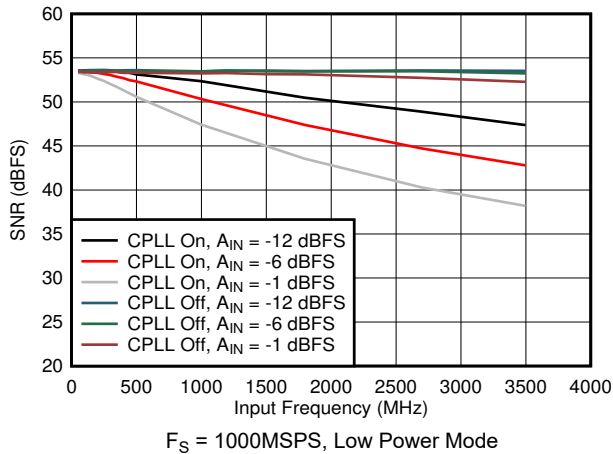
Figure 5-75. SNR vs Input Frequency, CPLL and Input Amplitude
