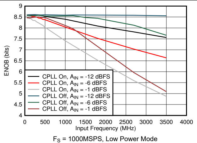
Figure 5-78. ENOB vs Input Frequency, CPLL and Input Amplitude
