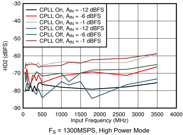
Figure 5-73. HD2 vs Input Frequency, CPLL and Input Amplitude
