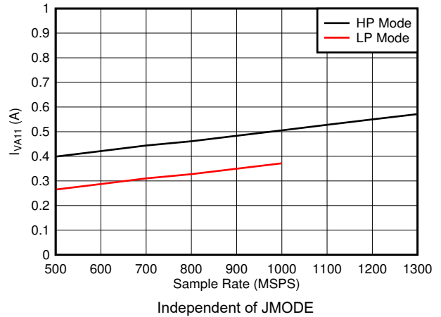
Figure 5-86. Quad Channel, I_{VA11} vs FS
