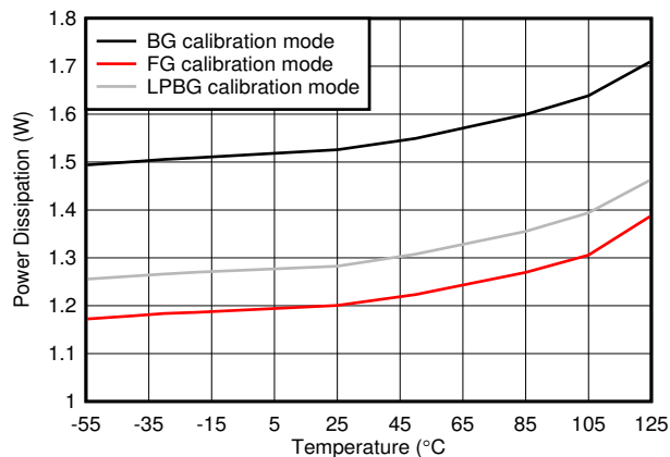
Figure 5-125. Single Channel, Power Dissipation vs Temperature
