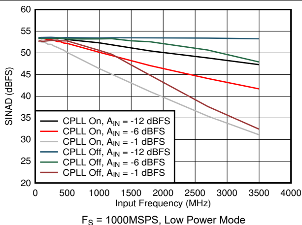
Figure 5-77. SINAD vs Input Frequency, CPLL and Input Amplitude
