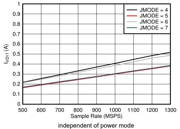
Figure 5-88. Quad Channel, I_{VD11} vs FS and JMODE 4 - 7
