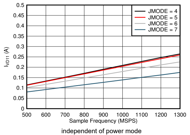
Figure 5-108. Single Channel, I_{VD11} vs FS and JMODE 4 - 7
