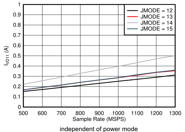
Figure 5-90. Quad Channel, I_{VD11} vs FS and JMODE 12 - 15
