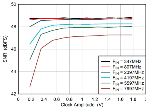
Figure 5-83. Dual Channel Mode: SNR vs Clock Amplitude
