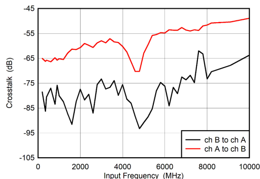
Figure 5-2. Crosstalk vs Input Frequency
