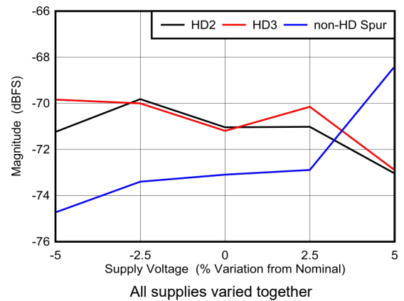
Figure 5-94. DES Mode: HD2, HD3 and Worst Spur vs Supply Voltage
