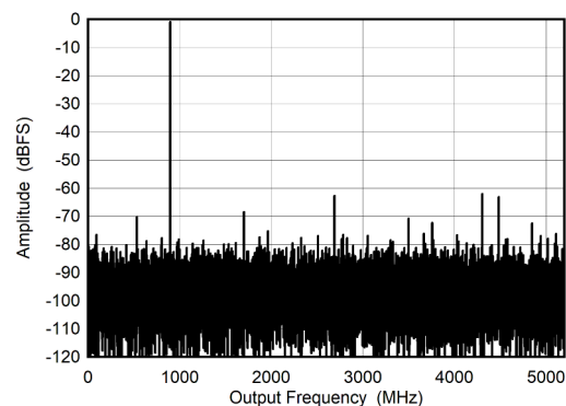
Figure 5-6. DES Mode: Single Tone FFT at 897 MHz
