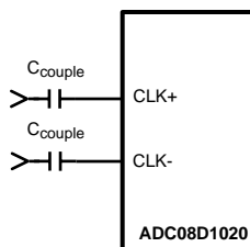
Figure 46. Differential (LVDS) Input Clock Connection
