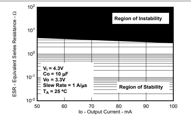
Figure 5-57. Typical Region of Stability ESR vs Output Current (New Chip)
