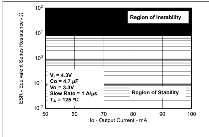
Figure 5-54. Typical Region of Stability ESR vs Output Current (New Chip)
