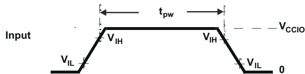
Figure 6-3. TTL-Level Inputs
