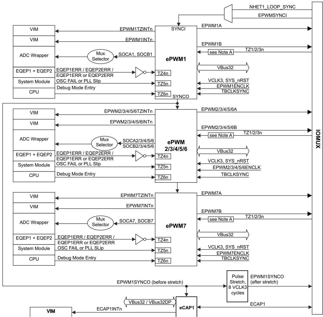
Figure 8-1. ePWMx Module Interconnections
