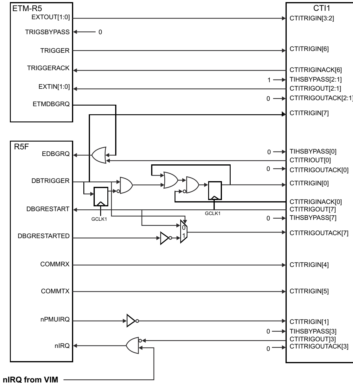
Figure 7-25. CTI1 Mapping
