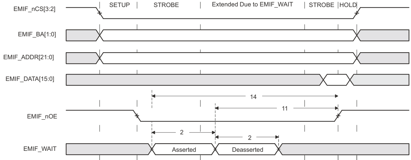
Figure 7-12. EMIFnWAIT Read Timing Requirements
