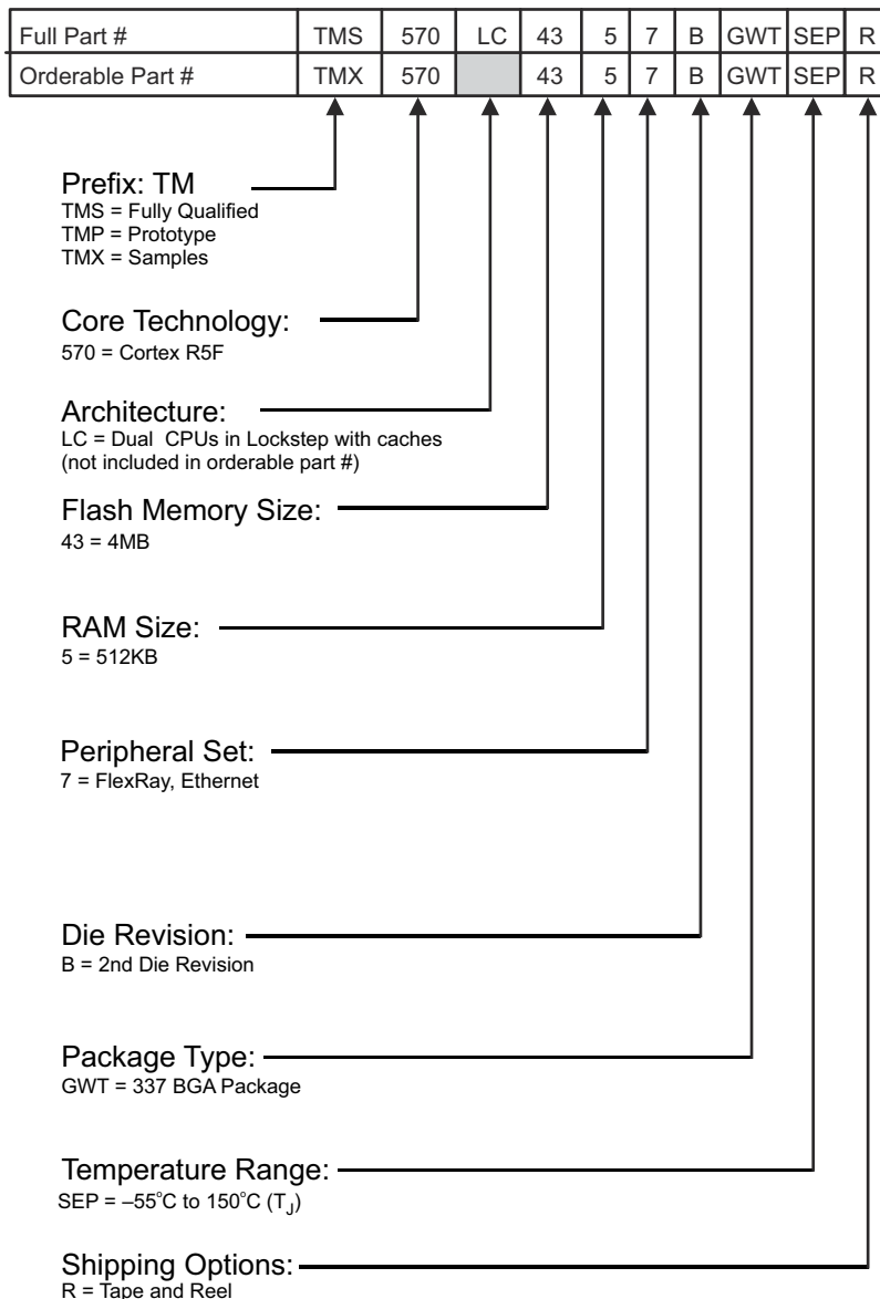
Figure 10-1. TMS570LC4357-SEP Device Numbering Conventions
