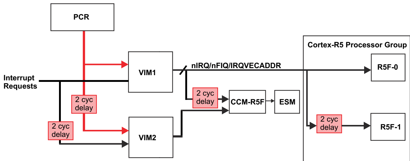
Figure 7-17. Interrupt Generation
