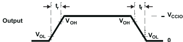
Figure 6-5. CMOS-Level Outputs
