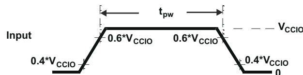
Figure 8-18. FlexRay Inputs
