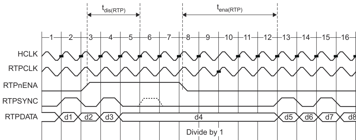
Figure 7-34. RTPnENA timing
