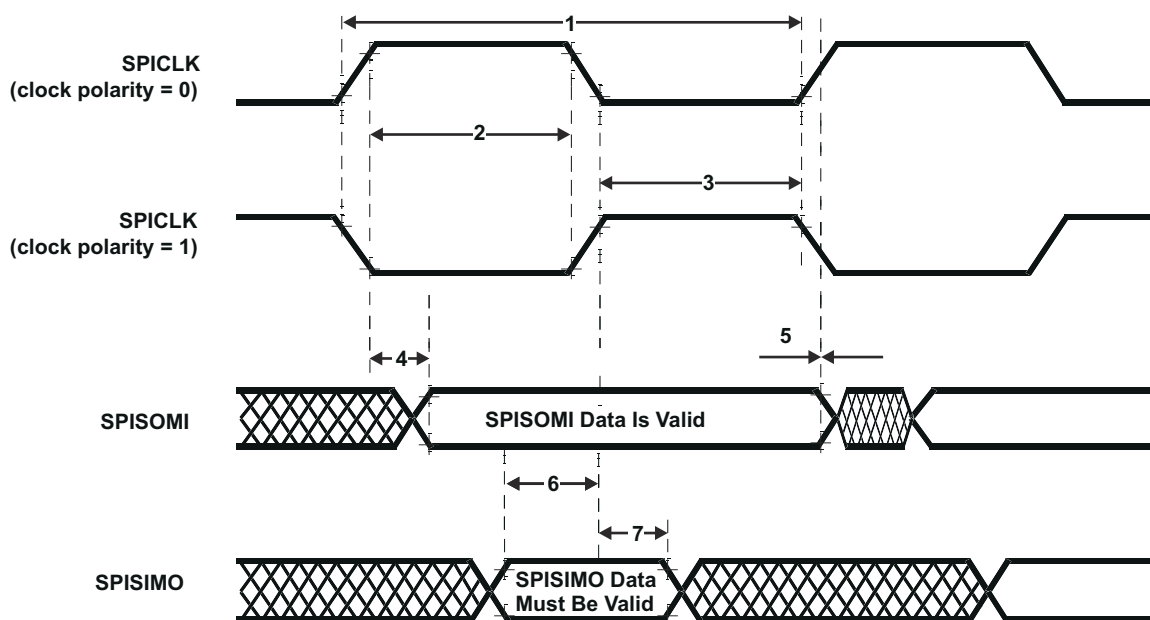
Figure 8-24. SPI Slave Mode External Timing (CLOCK PHASE = 0)
