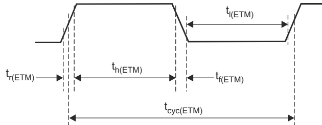
Figure 7-30. ETMTRACECLKOUT Timing
