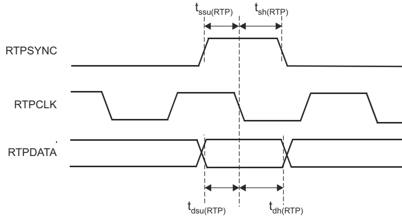
Figure 7-33. RTPDATA Timing
