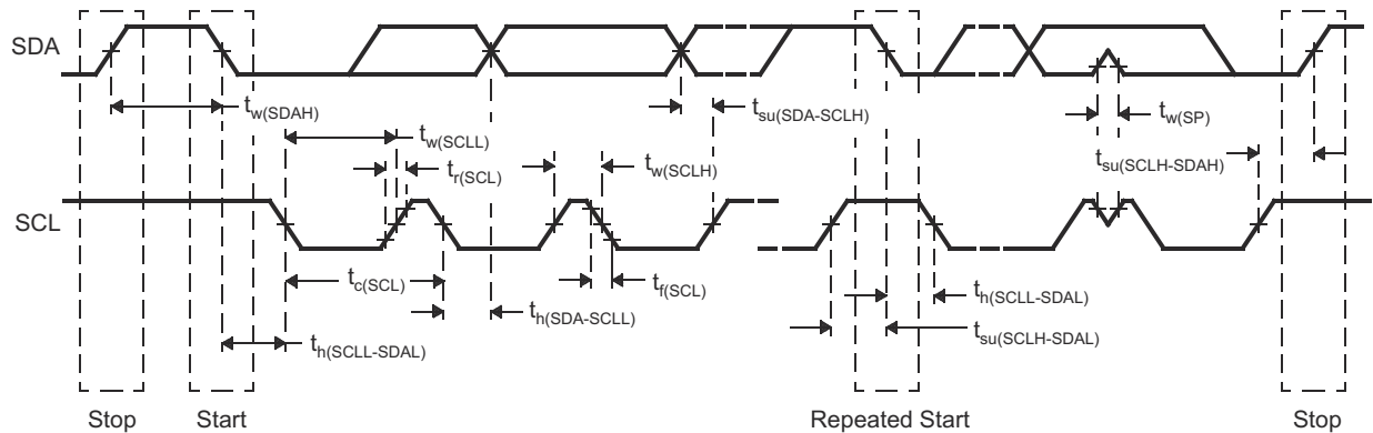
Figure 8-19. I2C Timings
