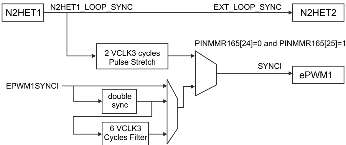
Figure 8-4. Synchronizing Time Bases Between N2HET1, N2HET2 and ePWMx Modules
