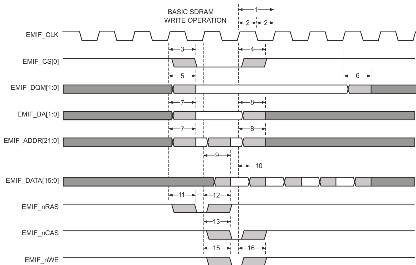
Figure 7-16. Basic SDRAM Write Operation
