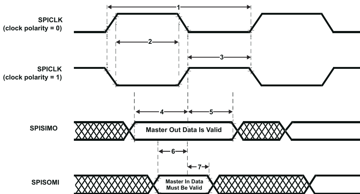
Figure 8-20. SPI Master Mode External Timing (CLOCK PHASE = 0)
