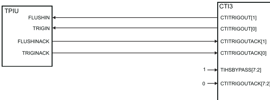
Figure 7-26. CTI3 Mapping
