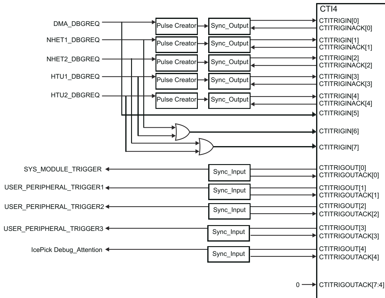
Figure 7-27. CTI4 Mapping
