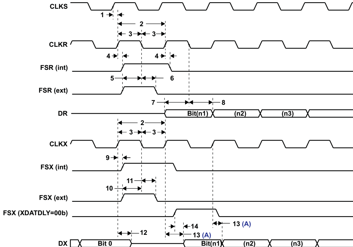
Figure 6-34. McBSP Timing
