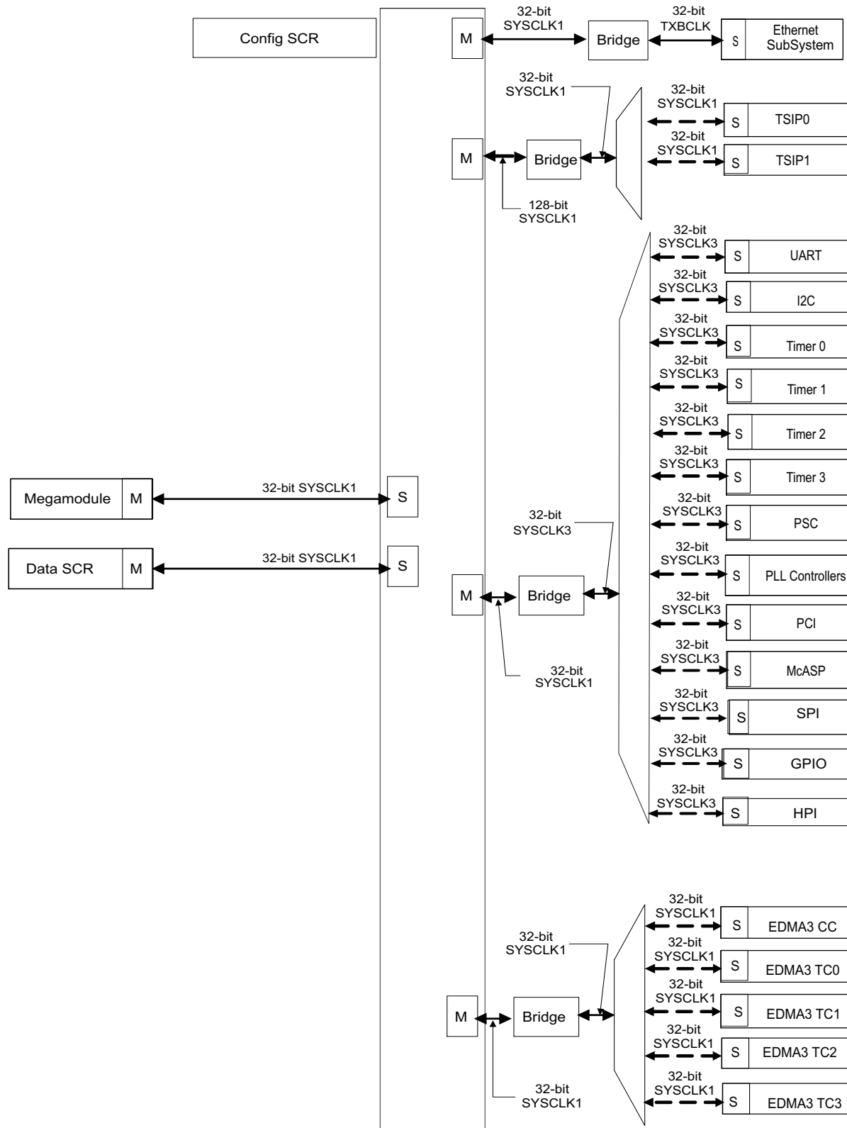
Figure 4-2. Configuration SCR
