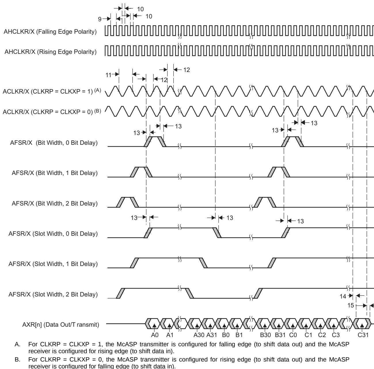
Figure 6-44. McASP Output Timing
