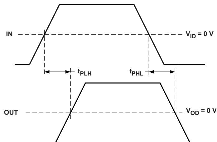
Figure 7-2. Propagation Delay Input to Output
