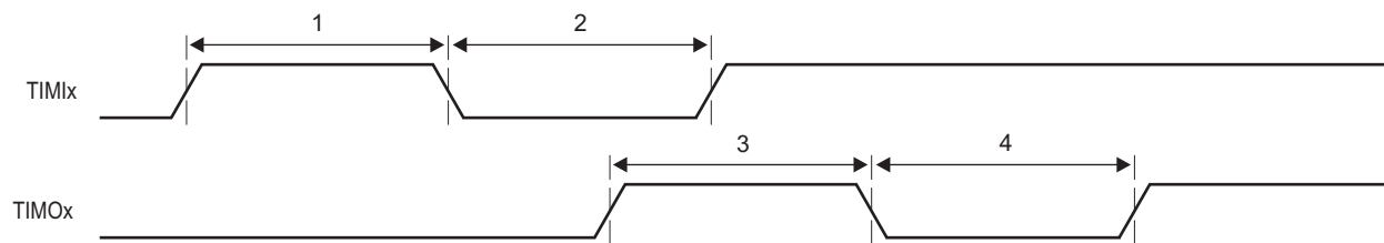
Figure 7-62 Timer Timing
