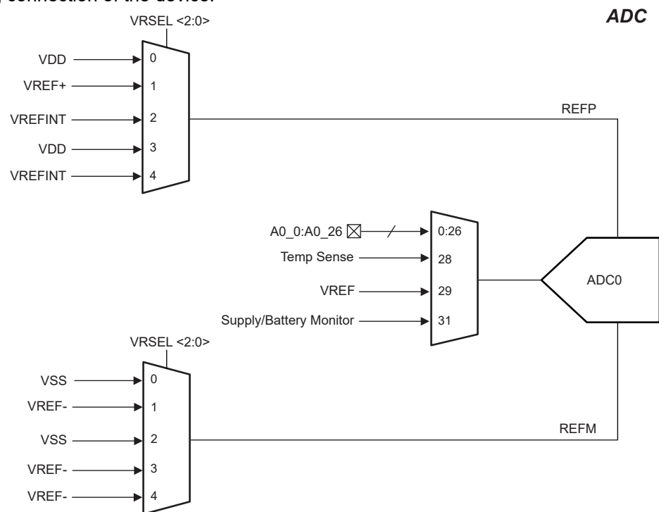
Figure 8-1. Analog Connections
