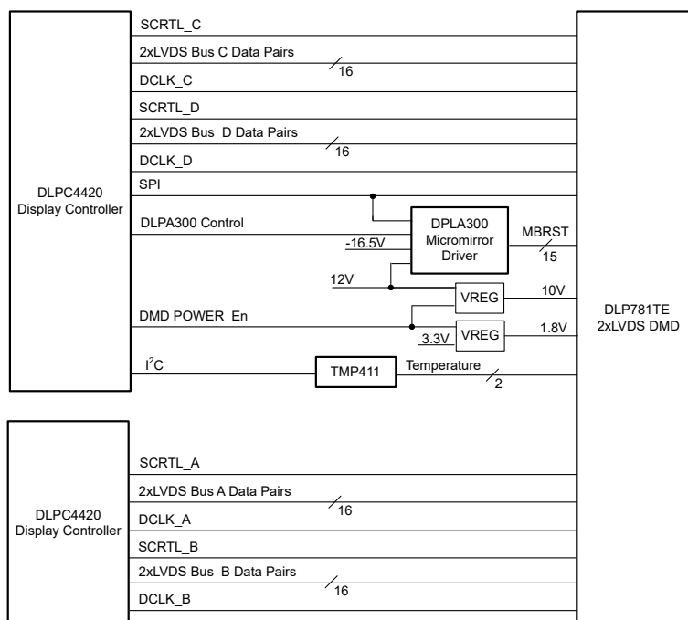
Simplified Application
