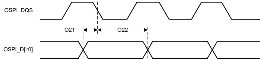
Figure 6-35. OSPI0 Timing Requirements – PHY SDR with External Board Loopback
