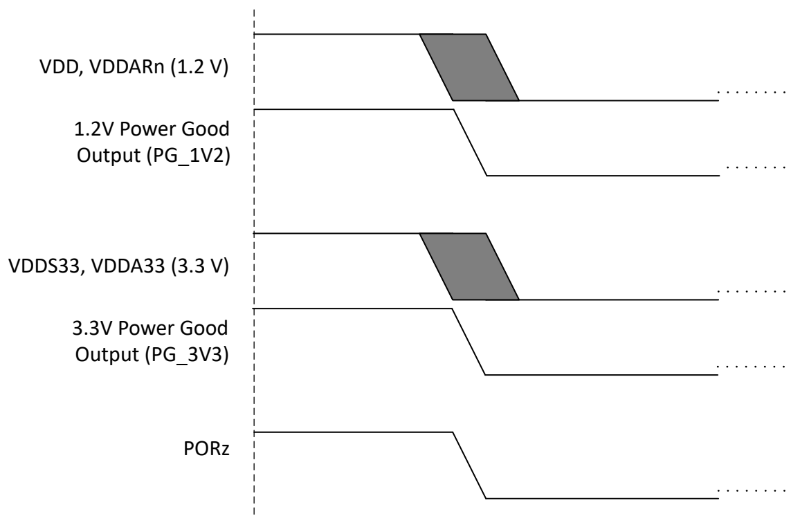
Figure 6-3. Power-Down Sequencing
