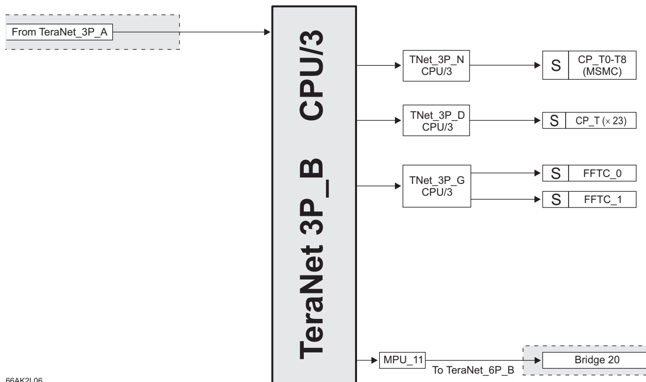
Figure 8-7. TeraNet 3P_B
