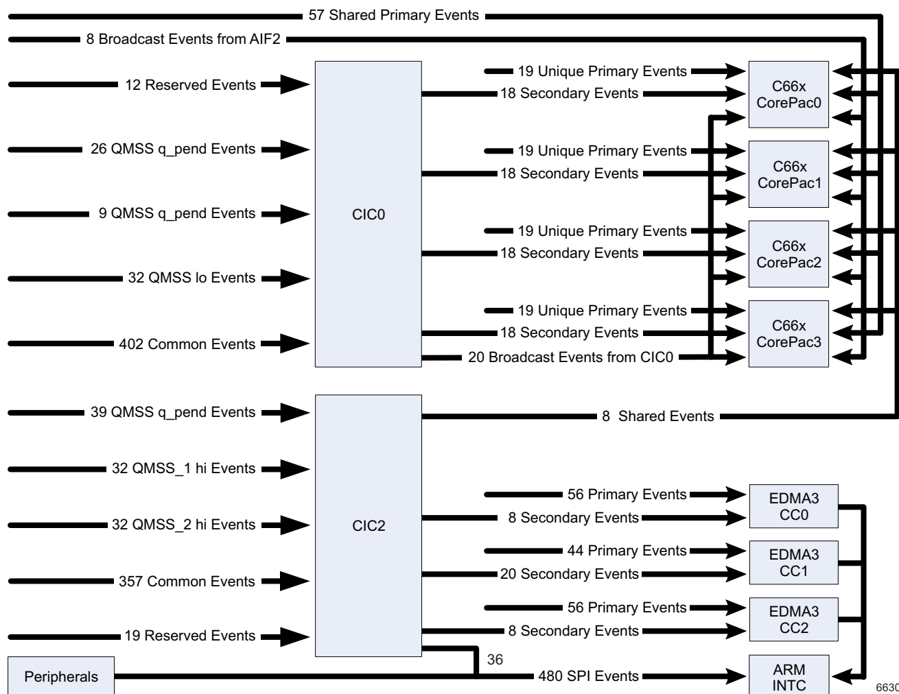
Figure 7-5. Interrupt Topology
