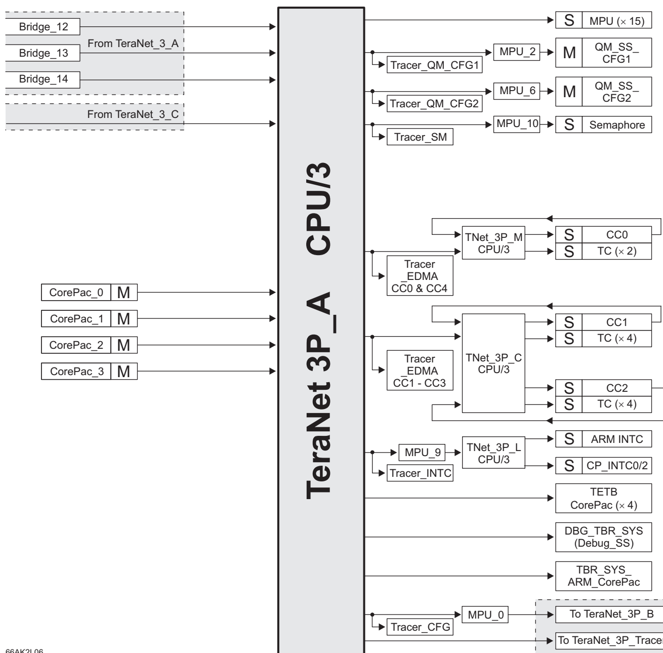
Figure 8-6. TeraNet 3P_A
