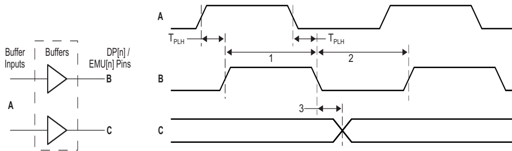
Figure 11-68. Trace Timing
