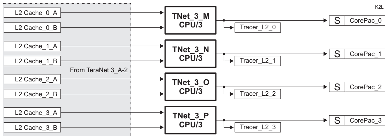
Figure 8-5. TeraNet C66x to SDMA
