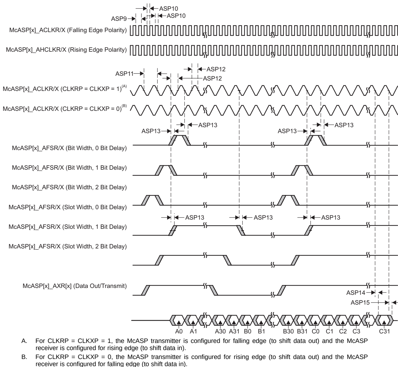
Figure 5-50. McASP Output Timing
