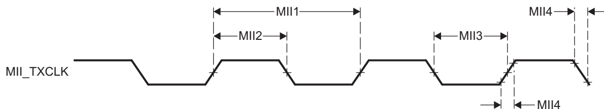
EMAC_MII_02
