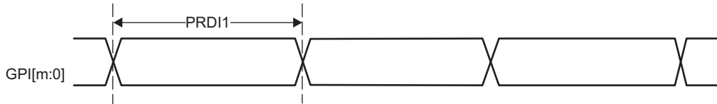
Figure 5-62. PRU-ICSS PRU Direct Input Timing
