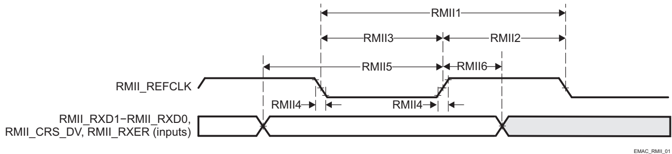
Figure 5-30. EMAC Receive Interface Timing RMI operation
