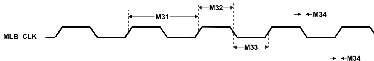
Figure 5-53. MLB_CLK Timing
