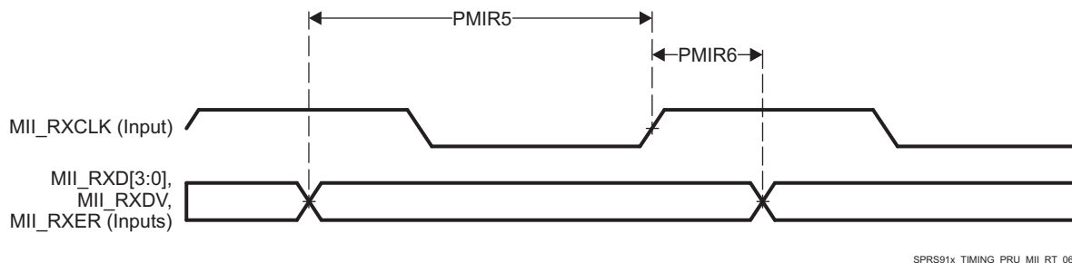
Figure 5-76. PRU-ICSS MII_RXD[3:0], MII_RXDV, and MII_RXER Timing
