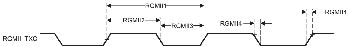
Figure 5-33. RGMII_TCX Timing - RGMII Mode
