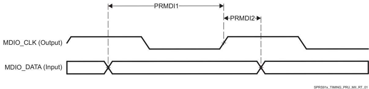
Figure 5-71. PRU-ICSS MDIO_DATA Timing – Input Mode
