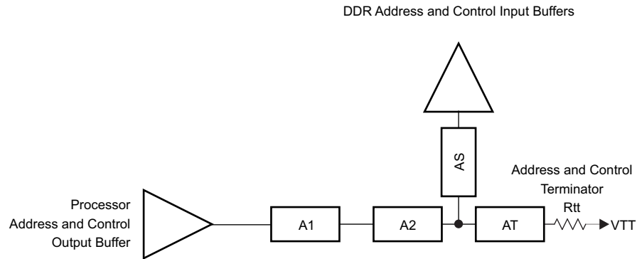
Figure 7-13. ADDR_CTRL Topology for One DDR3L Device
