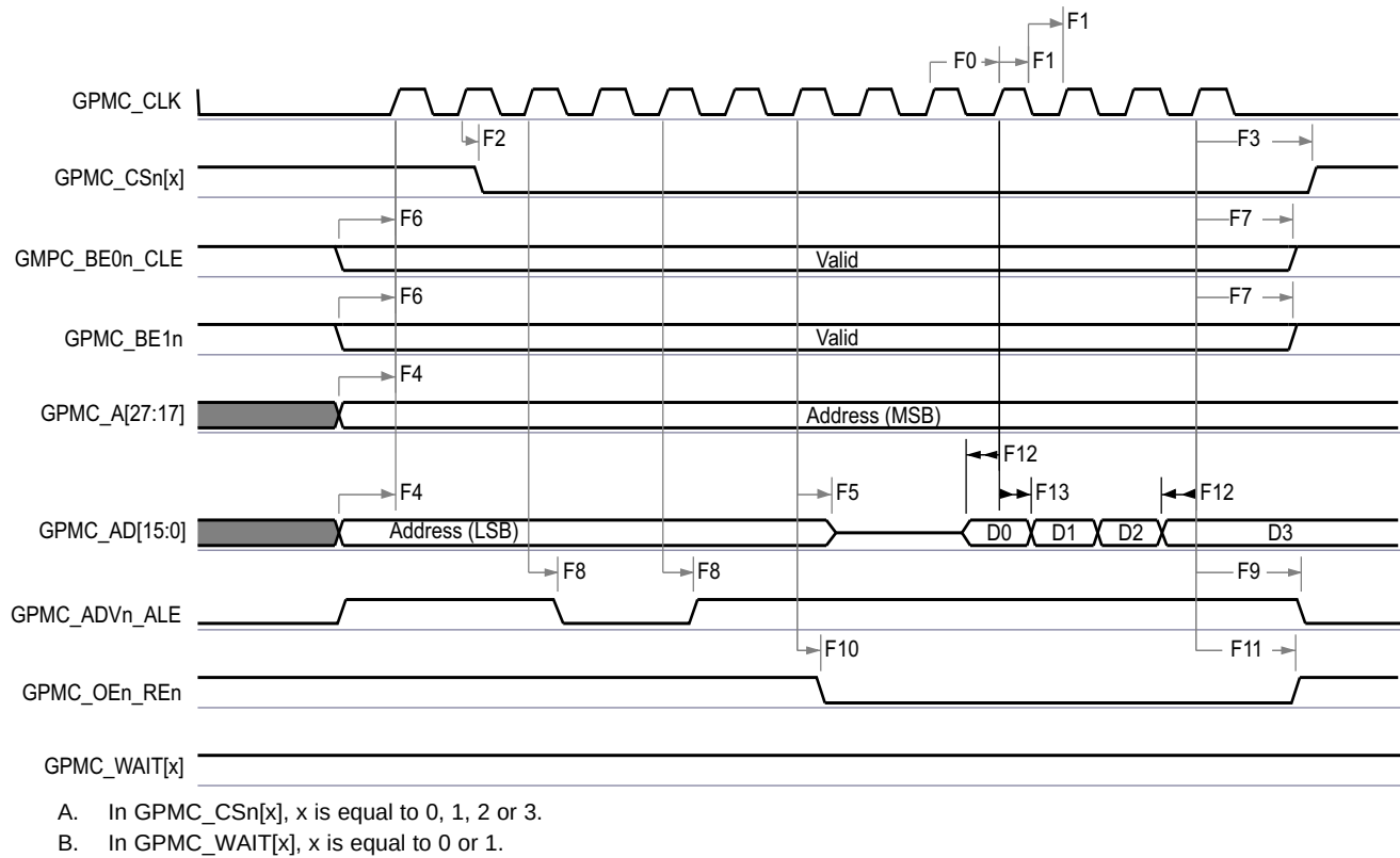
Figure 5-39. GPMC and Multiplexed NOR Flash—Synchronous Burst Read
