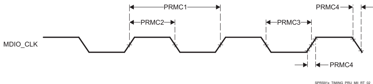
Figure 5-72. PRU-ICSS MDIO_CLK Timing
