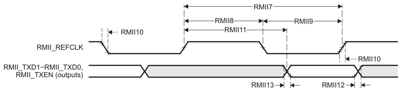
Figure 5-31. EMAC Transmit Interface Timing RMI Operation
