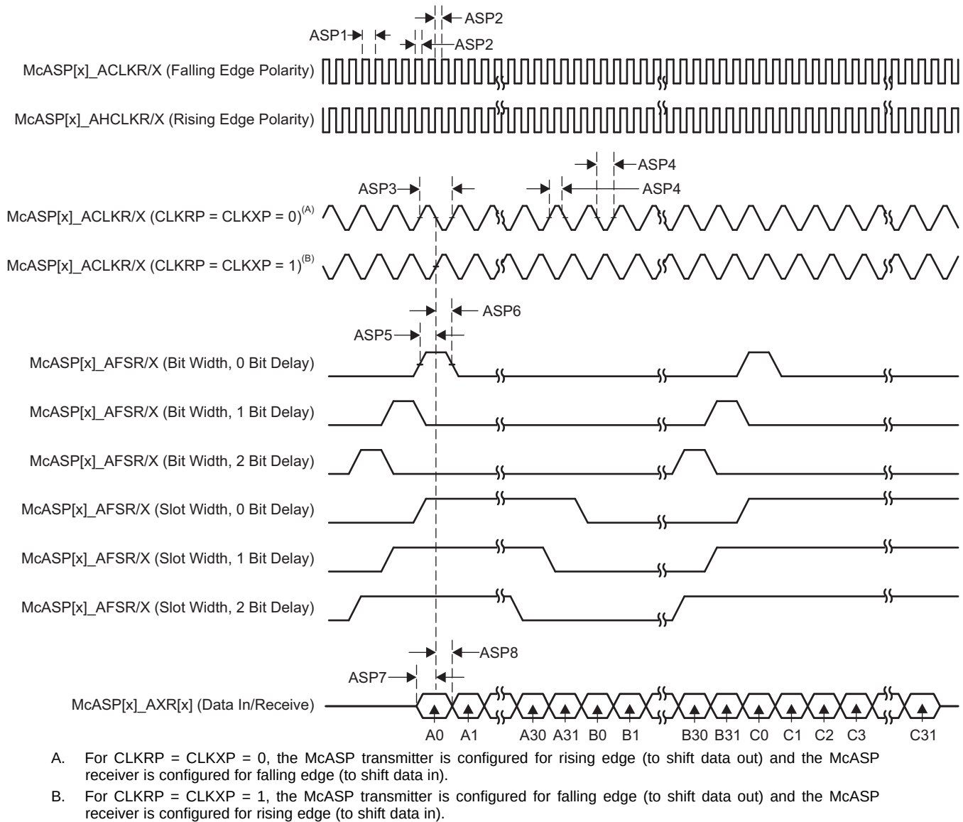
Figure 5-49. McASP Input Timing
