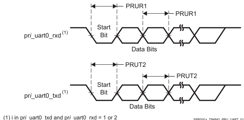
Figure 5-78. PRU-ICSS UART Timing
