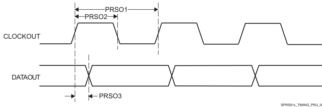
Figure 5-67. PRU-ICSS PRU Shift Out Timing
