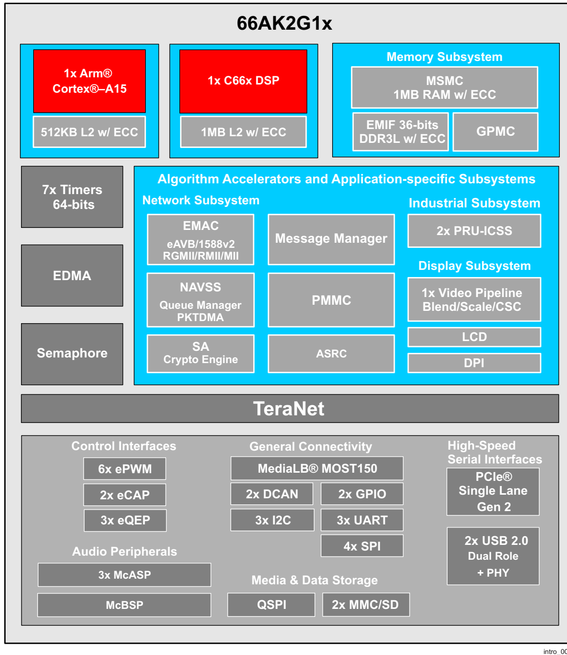
Figure 6-1. Functional Block Diagram
