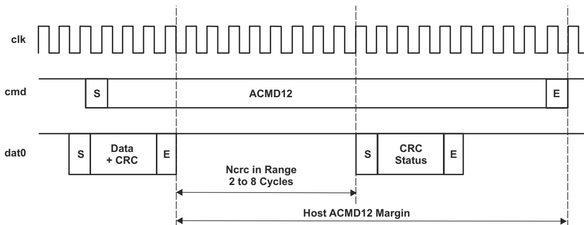
Figure 20-18. Auto CMD12 Timing During Write Transfer
