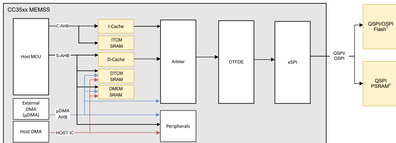
Figure 8-1. CC35xx Memory Subsystem
