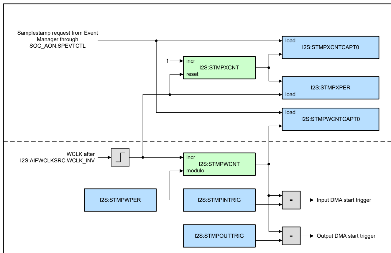
Figure 22-11. Samplestamp Generator
