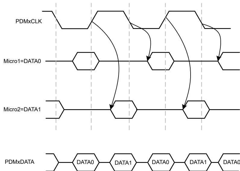
Figure 23-3. PDM Data Mode
