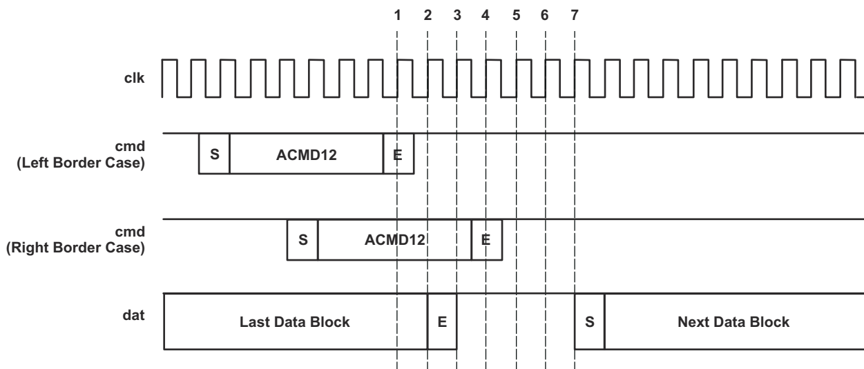
Figure 20-19. Auto Command 12 Timings During Read Transfer
