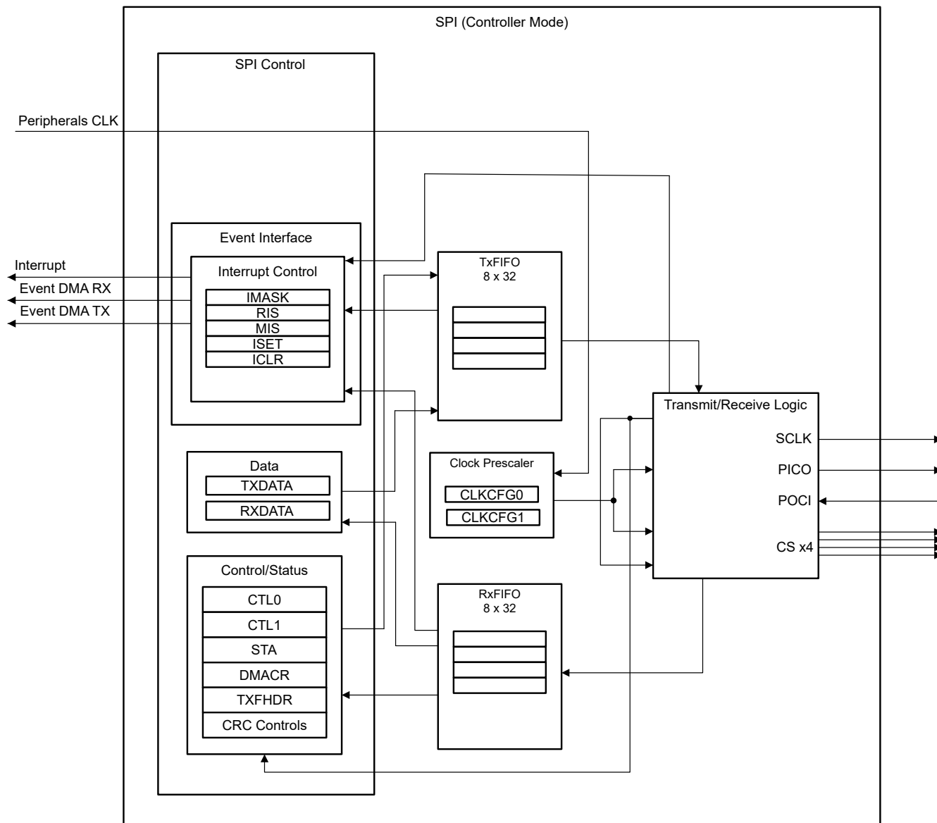
Figure 18-1. SPI Block Diagram
