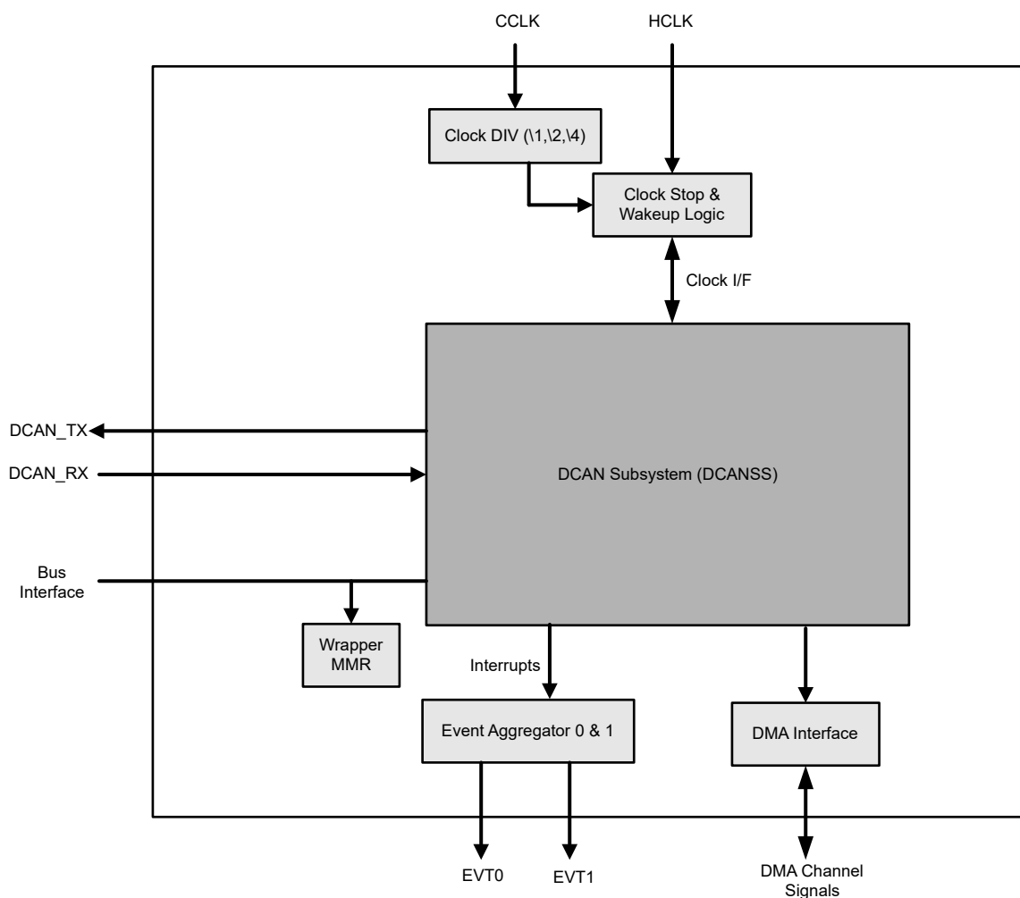
Figure 25-13. DCAN Wrapper
