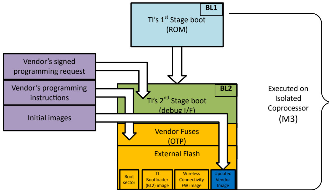
Figure 10-5. Reprogramming Flow
