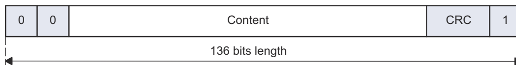
Figure 20-7. 136-Bit Response Packet (R2)
