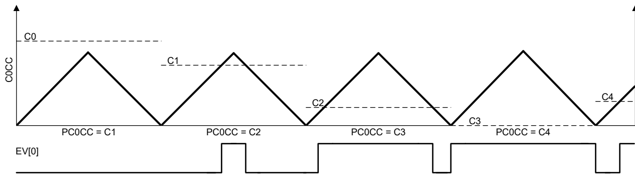
Figure 13-6. Center-Aligned PWM
