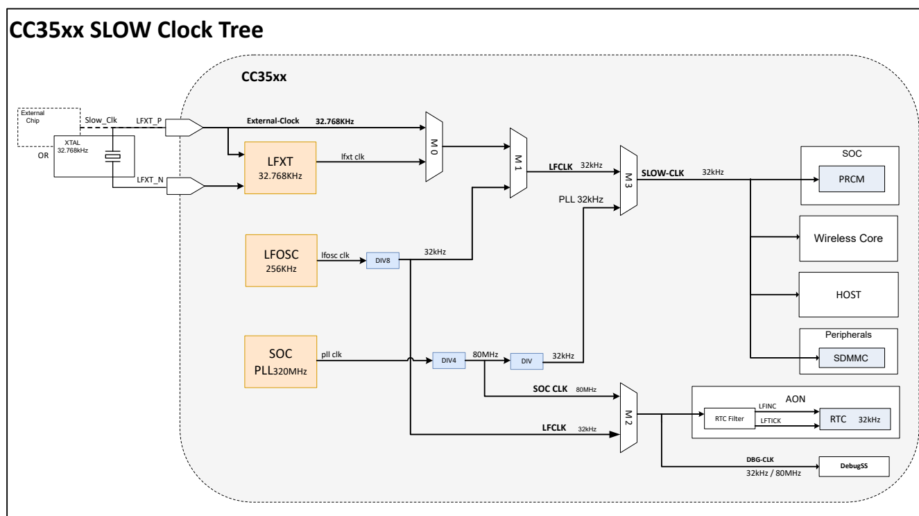
Figure 7-5. Slow Clock Tree
