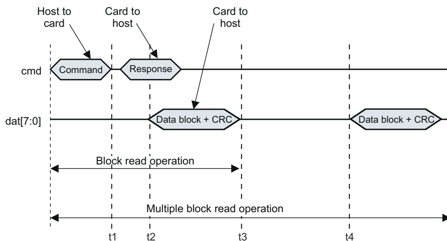
Figure 20-17. Read Data Timeout
