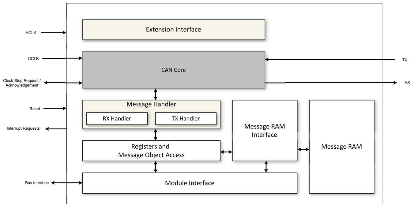
Figure 25-1. DCAN Block Diagram
