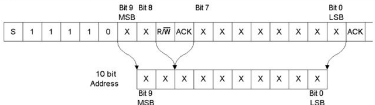
Figure 19-8. I2C 10-Bit Address Structure
