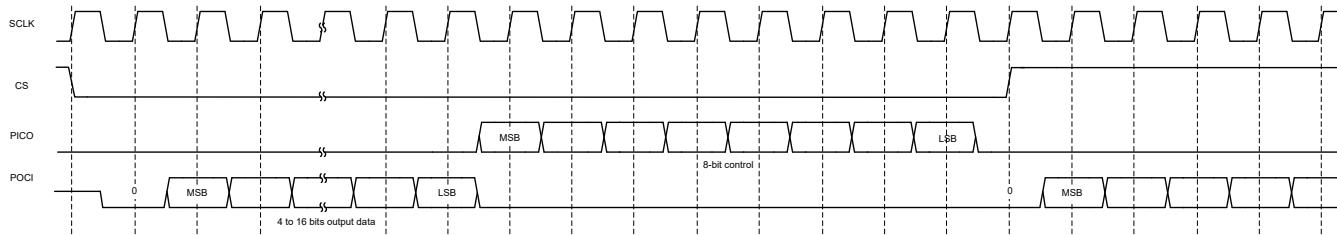
Figure 18-8. MICROWIRE Frame Format (Continuous Transfer)
