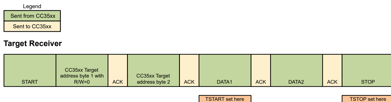
Figure 19-11. Target Reciever in 10-bit addressing
