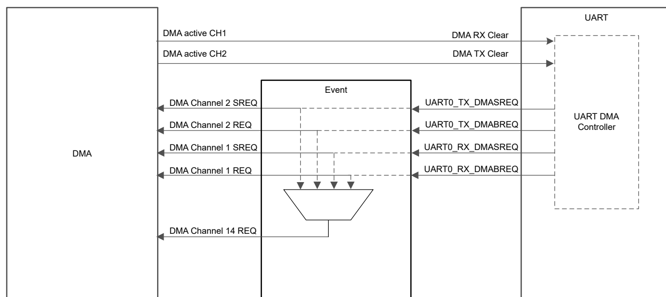
Figure 17-4. DMA Example
