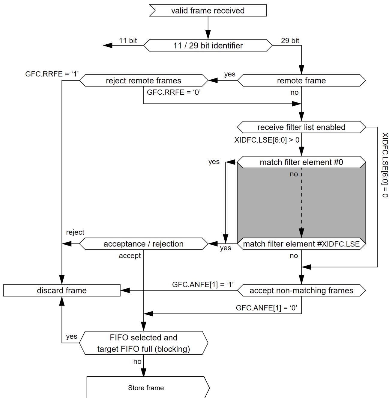
Figure 25-6. Extended Message ID Filter Path
