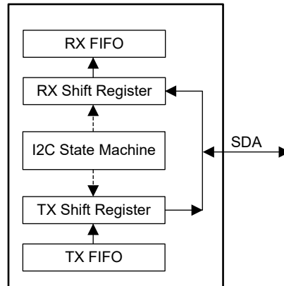
Figure 19-18. FIFO Operation
