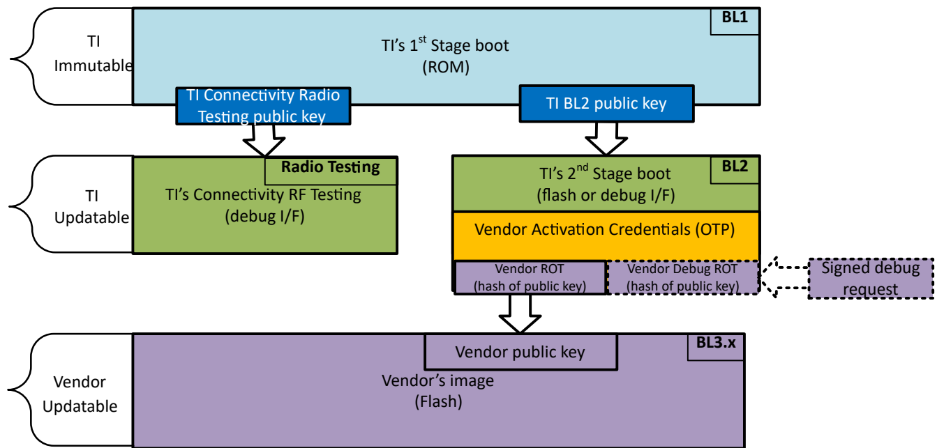
Figure 10-7. Chain of Trust
