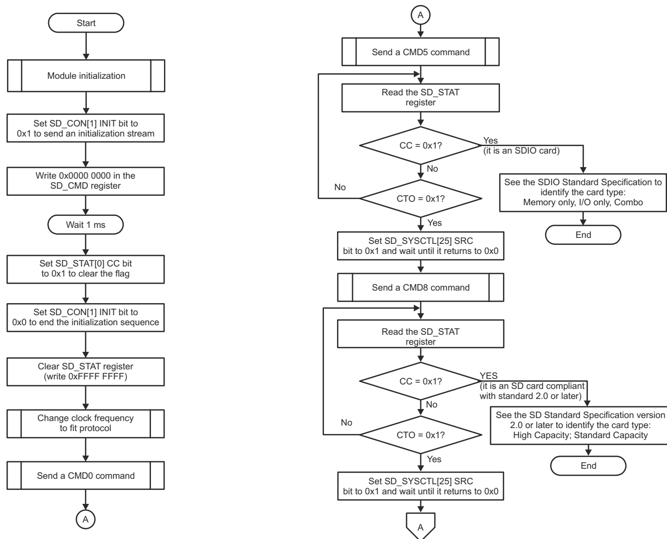
Figure 20-24. SD Card Identification and Selection - Part 1
