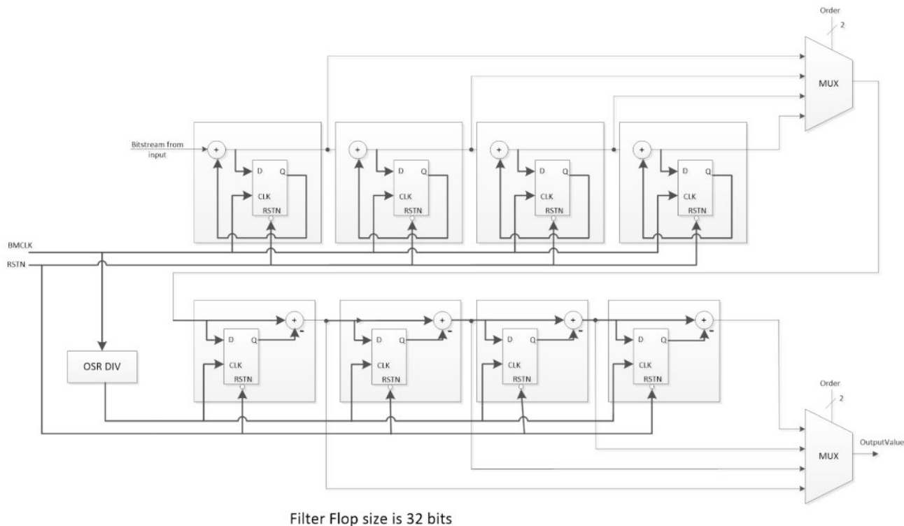
Figure 23-5. CIC Filter
