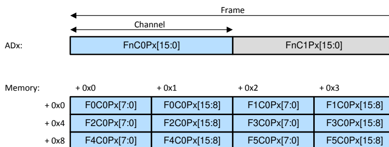
Figure 22-8. 16-Bit Mono I 2 S, LJF, and RJF Formats on One ADx Pin, Showing Six Frames in Memory
