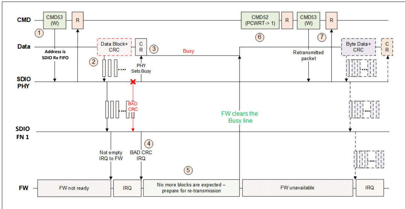
Figure 21-4. Host Write to SDIO with CRC Error
