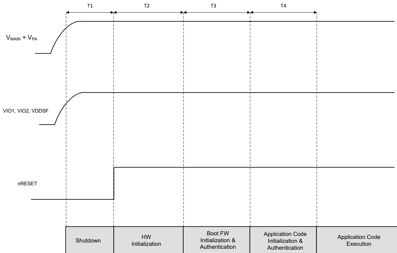
Figure 7-3. CC35xx Boot Sequence
