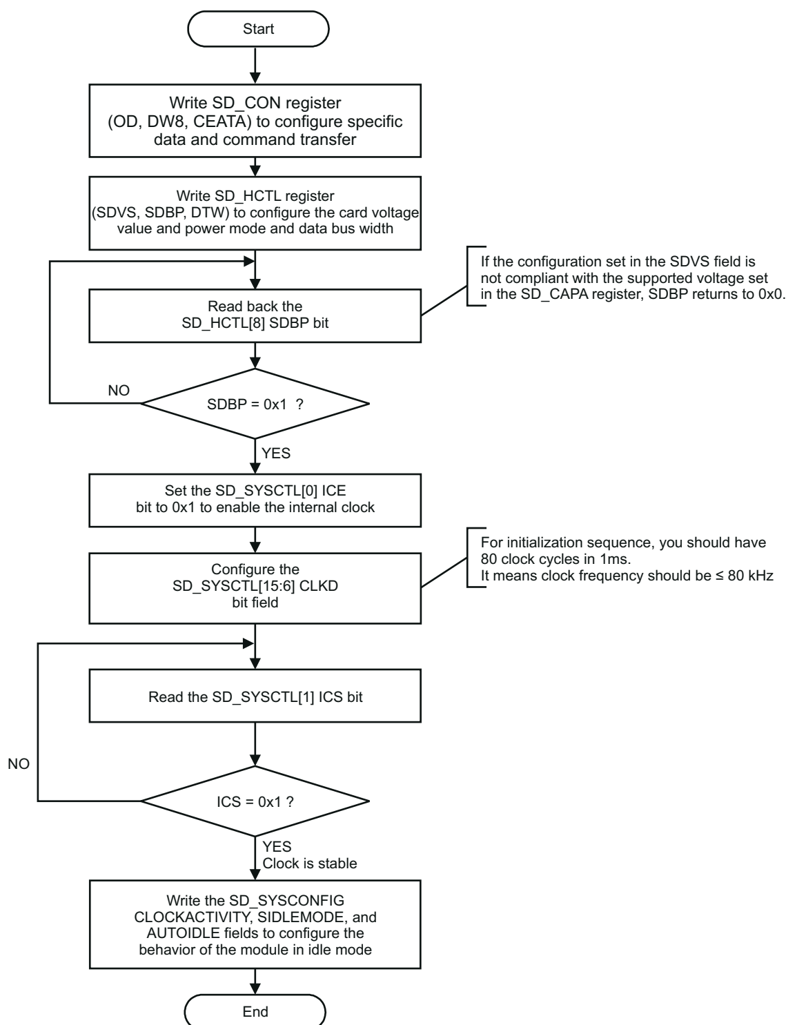
Figure 20-23. SDMMC Bus Configuration Flow
