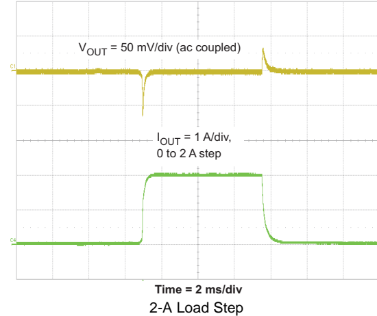
Figure 41. Transient Response
