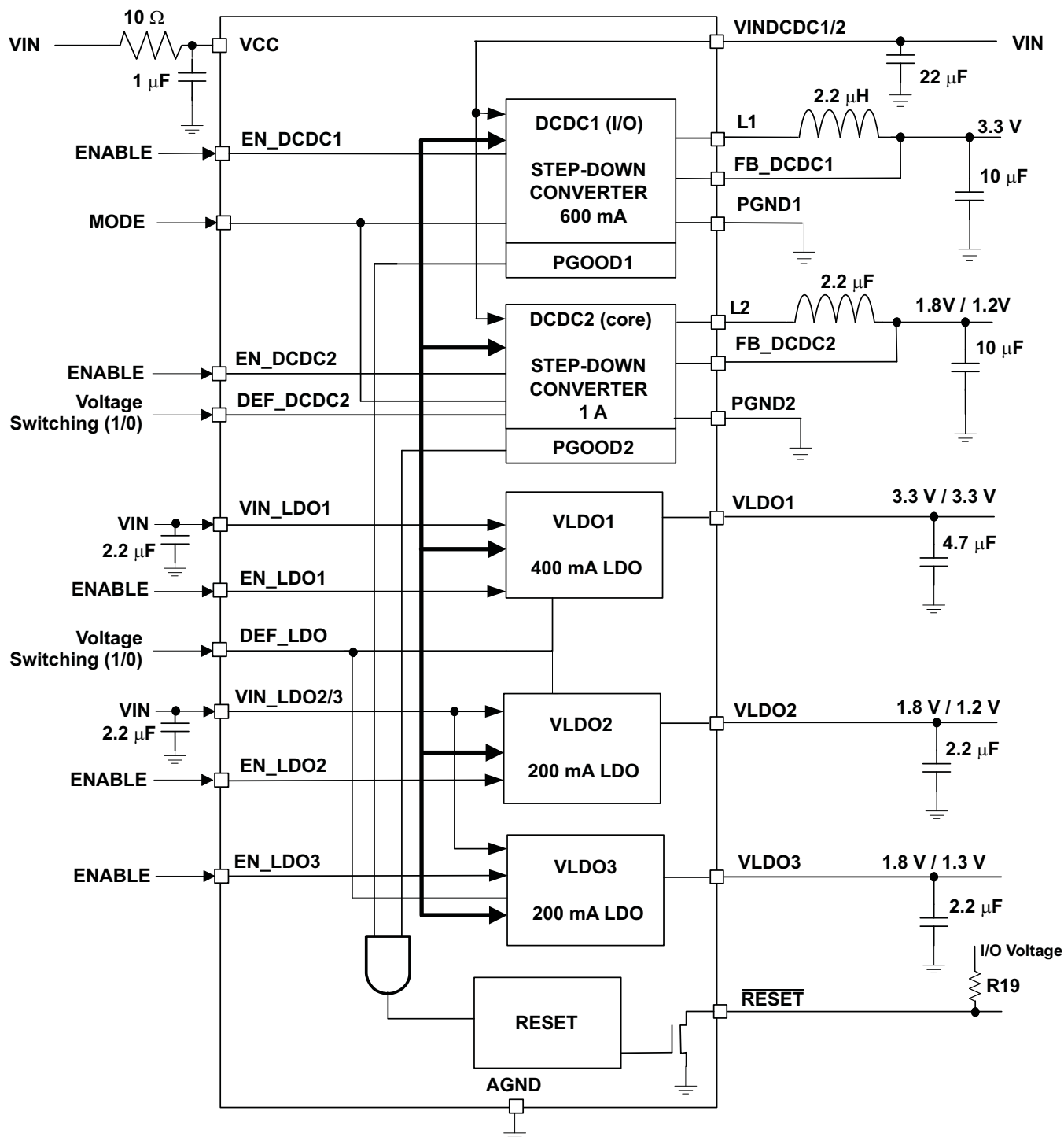
Figure 20. TPS65058 Functional Block Diagram
