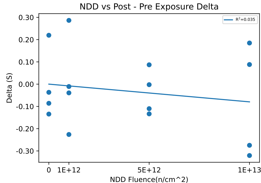
Test Statistics (S)
